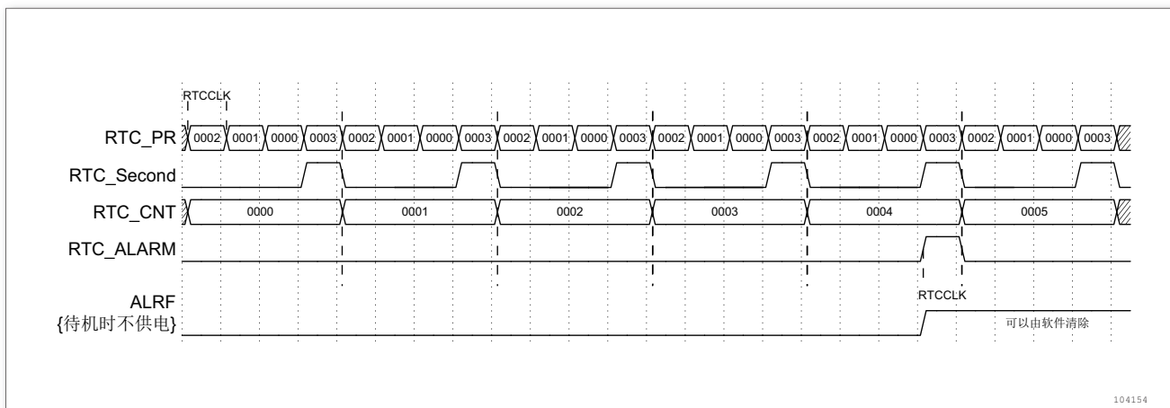
图 181. RTC 秒和闹钟波形图示例, PR = 0003, ALARM = 00004
