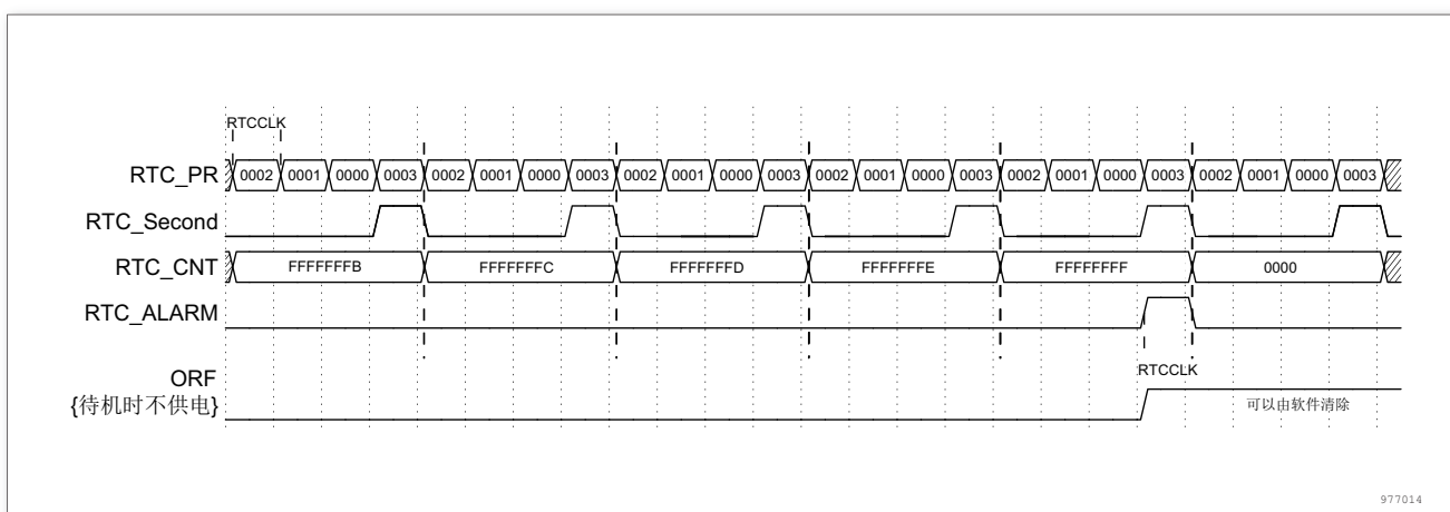
图 182. RTC 溢出波形图示例, PR = 0003
