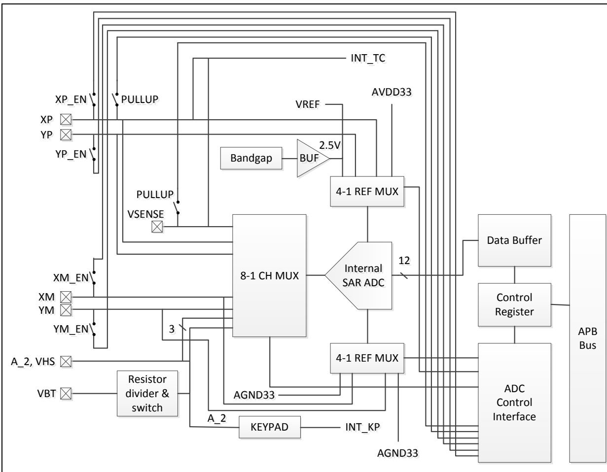
Figure 5.30-1 ADC Functional Block Diagram
