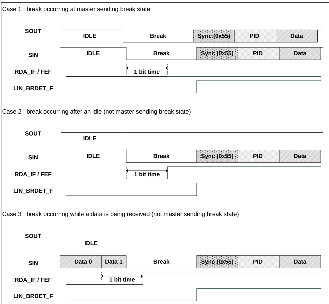
Figure 5.15-13 Relationship between Break Detection and Frame Error Detection
