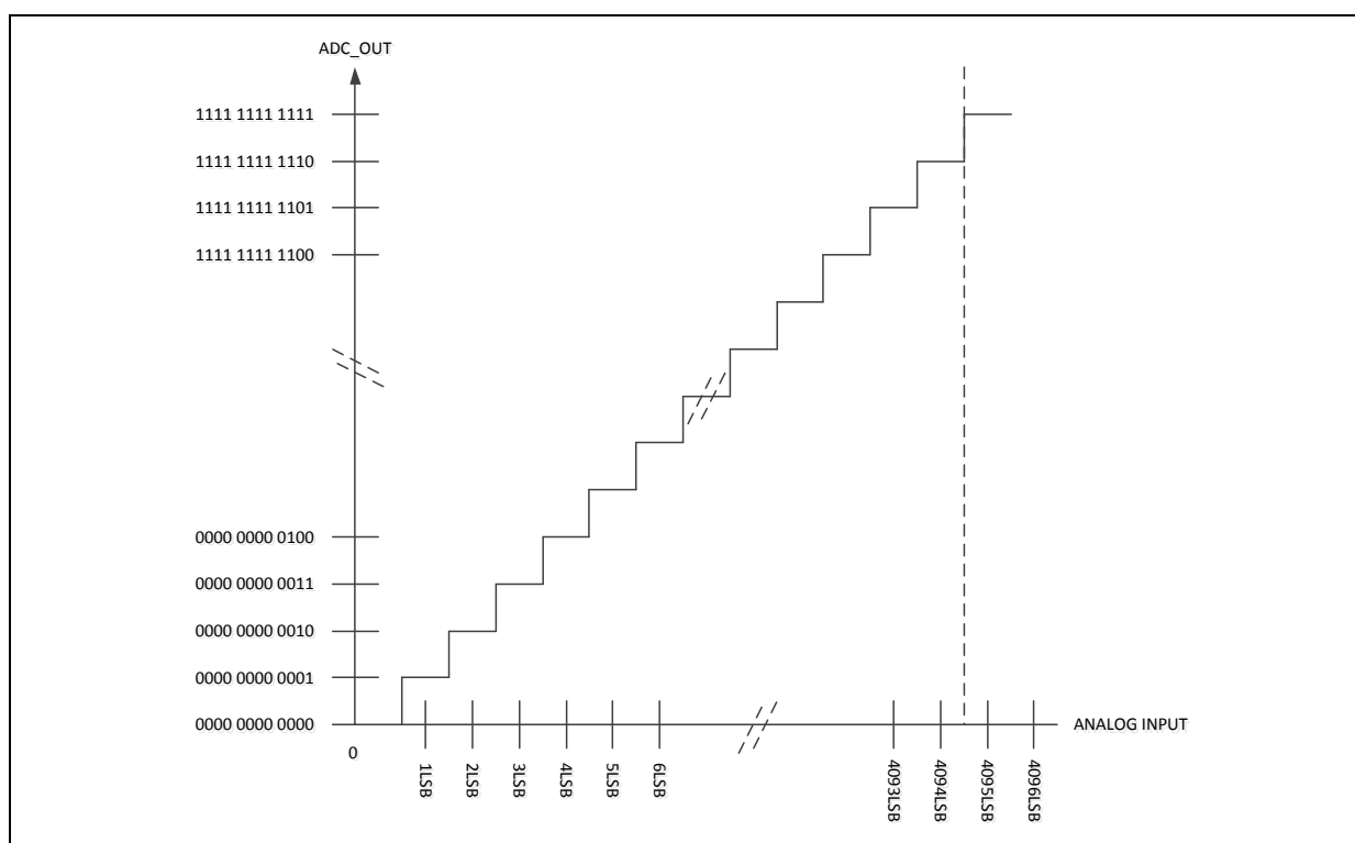
Figure 5.30-2 ADC Transfer Function
