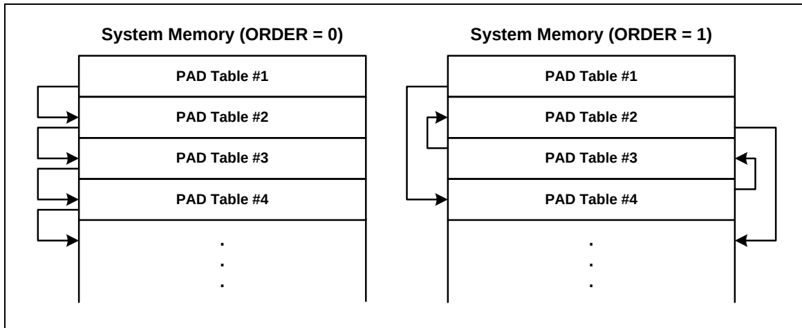
Figure 5.25-2 PAD (Physical Address Descriptor) Table Fetch Modes
