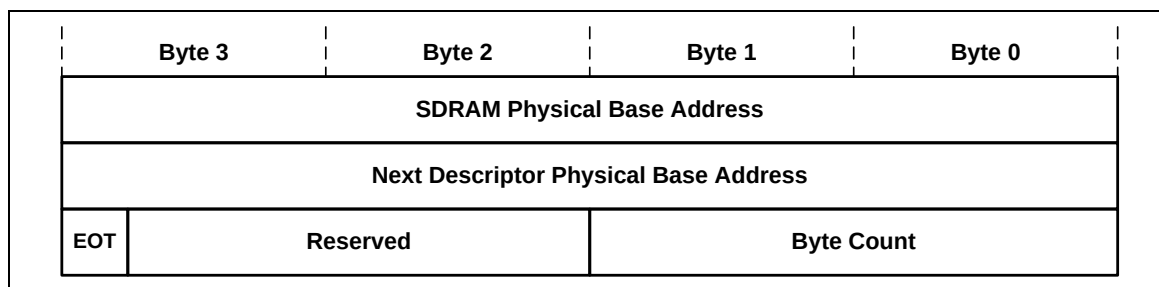
Figure 5.24-5 PAD (Physical Address Descriptor) Table Format
