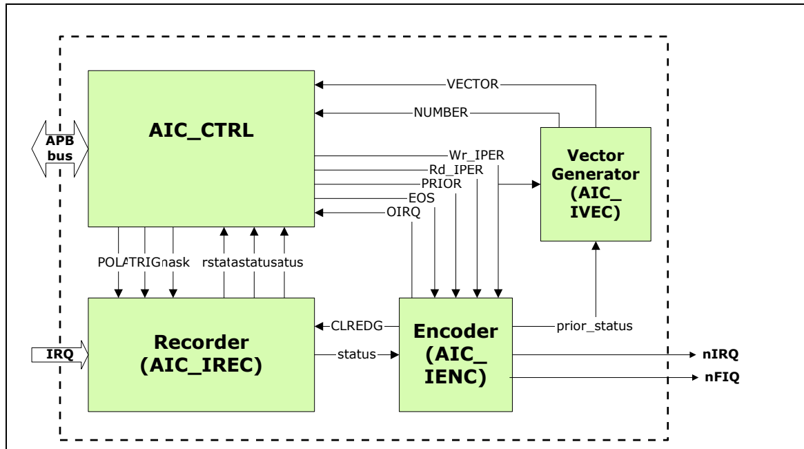
Figure 5.4-1 Advanced Interrupt Controller (AIC) Block Diagram
