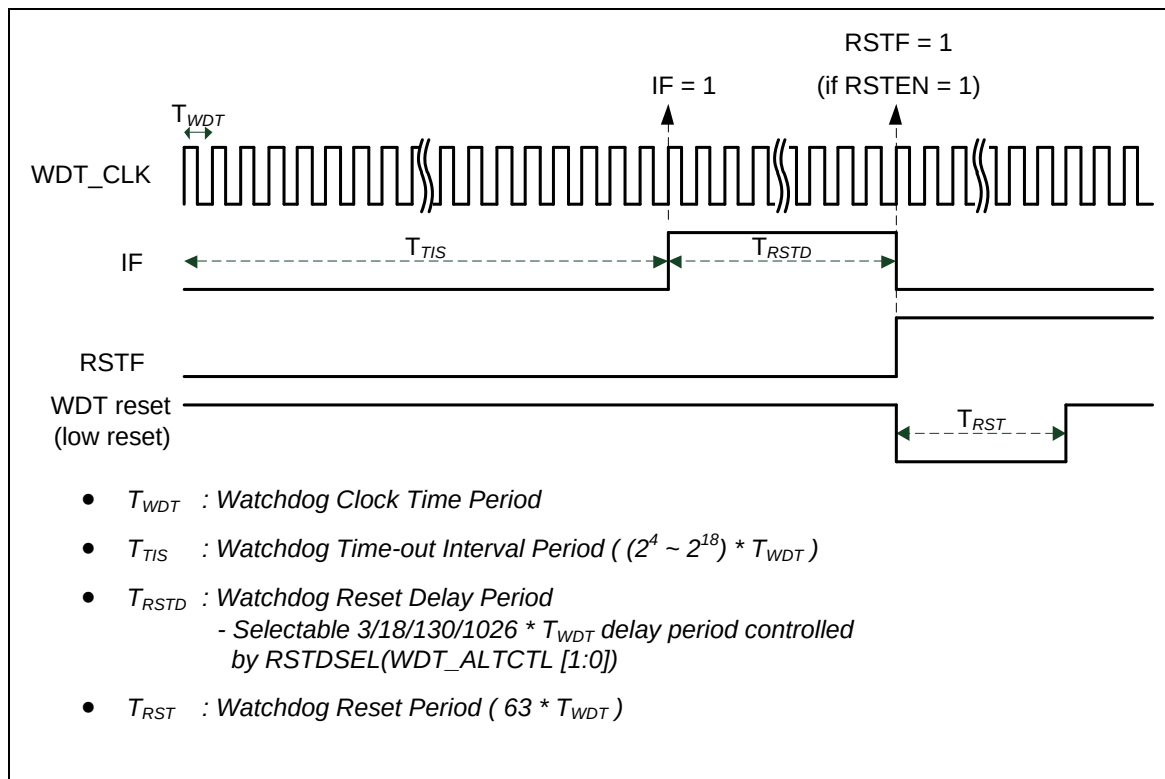
Figure 5.12-3 Watchdog Timer Time-out Interval and Reset Period Timing
