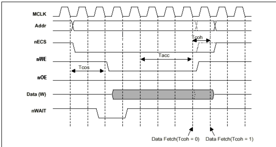
Figure 5.6-2 External I/O Write operation timing
