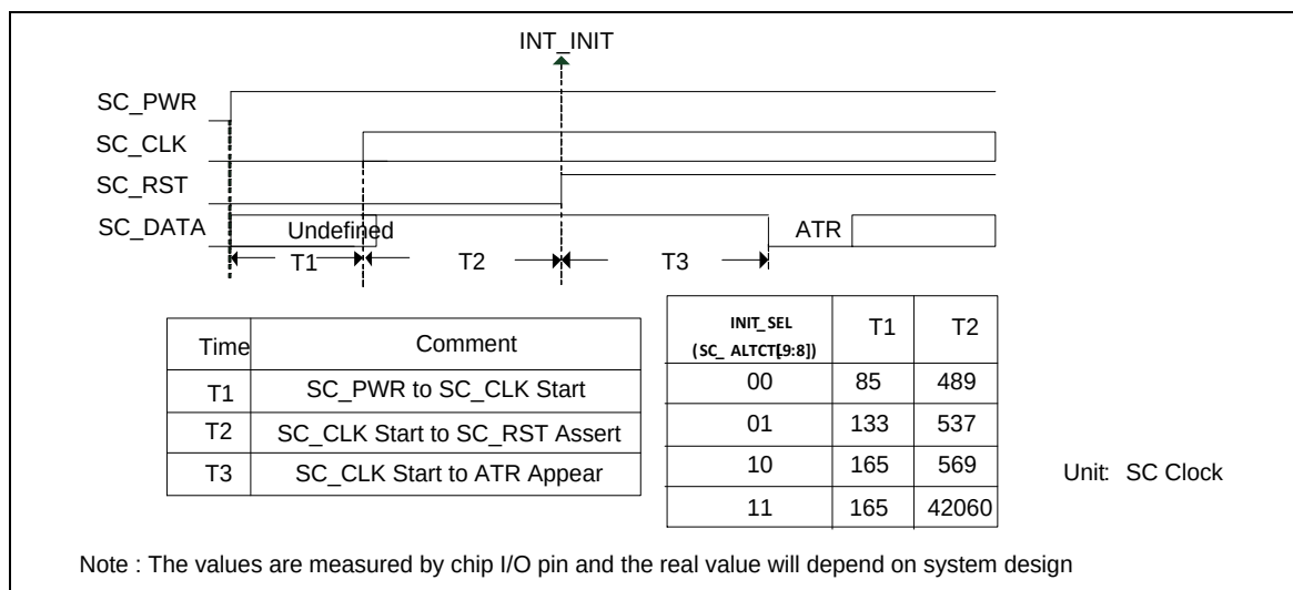
Figure 5.16-4 SC Activation Sequence
