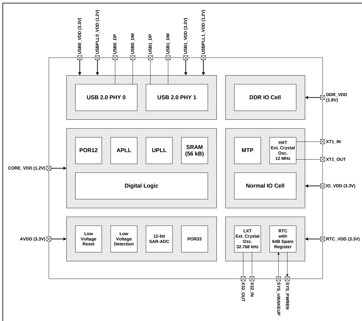
Figure 5.2-1 N9H30 Series Power Distribution Diagram
