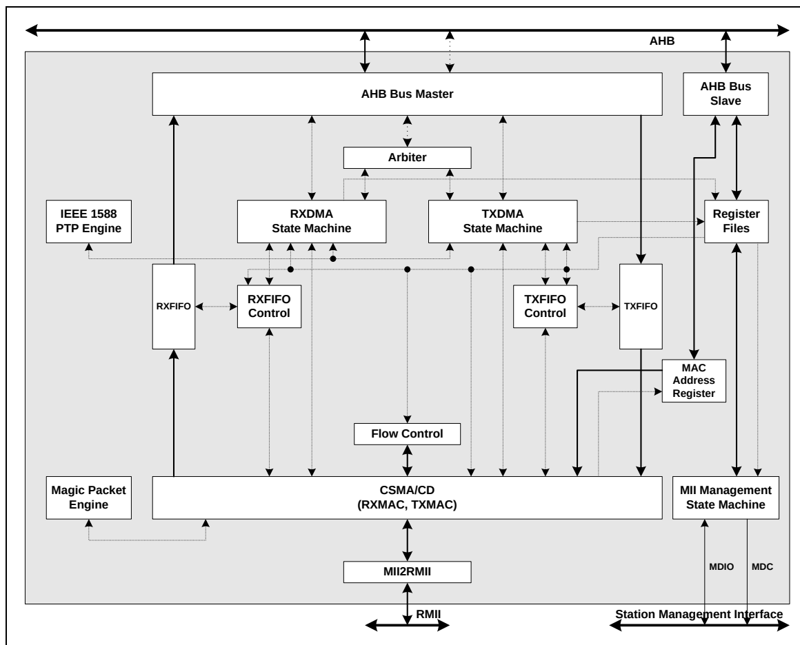
Figure 5.20-1 Ethernet MAC Controller Block Diagram
