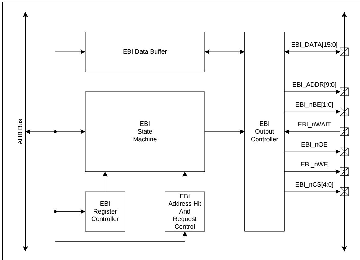
Figure 5.6-1 EBI Block Diagram
