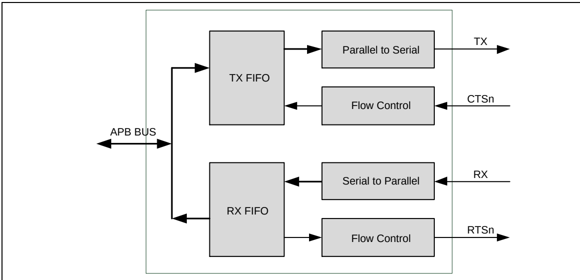
Figure 5.15-5 UART Auto-Flow Control Block Diagram
