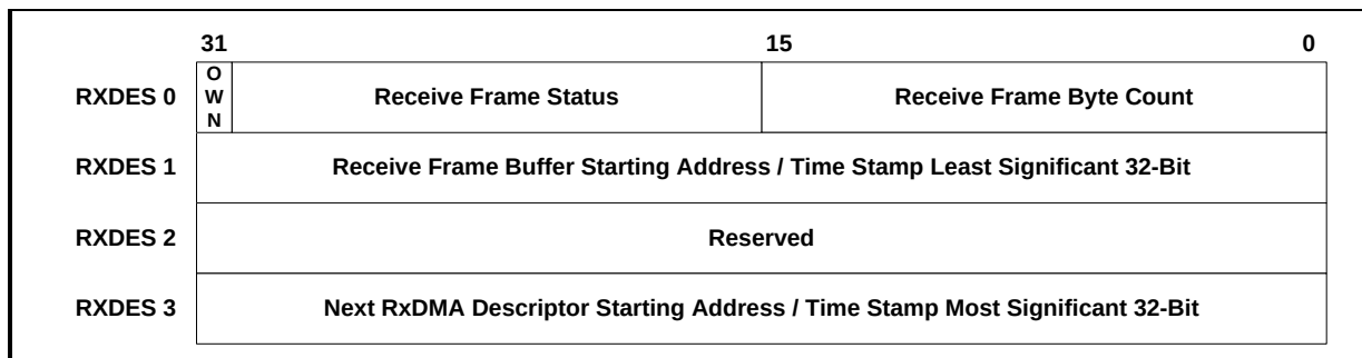
Figure 5.20-4 RXDMA Descriptor Data Structure
