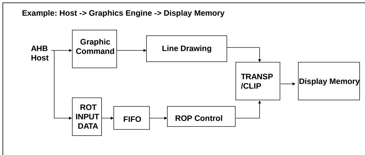
Figure 5.26-1 2-D GE Engine Architecture
