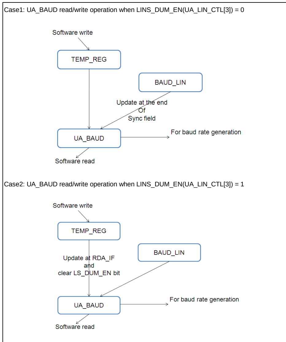
Figure 5.15-15 UA_BAUD Update Method
