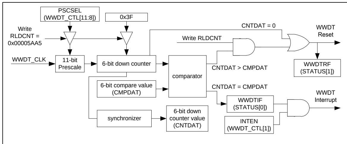
Figure 5.13-1 WWDT Block Diagram
