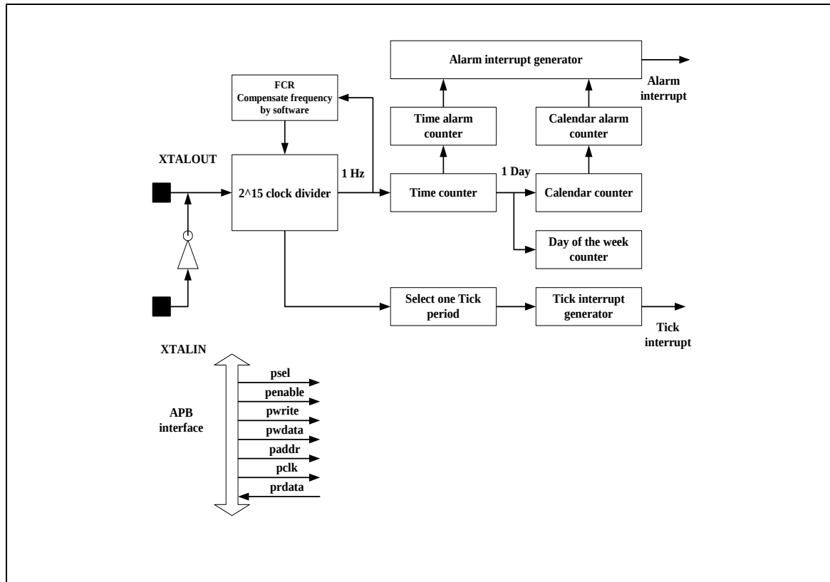
Figure 5.14-1 RTC Functional Block Diagram
