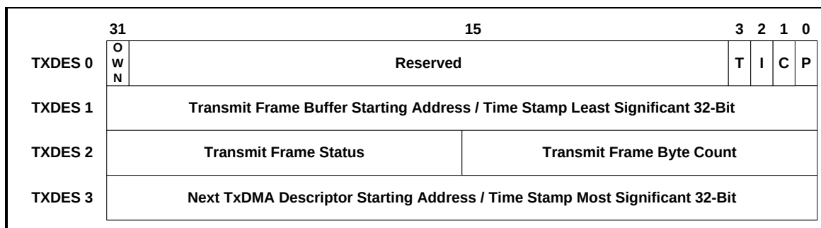
Figure 5.20-5 TXDMA Descriptor Data Structure
