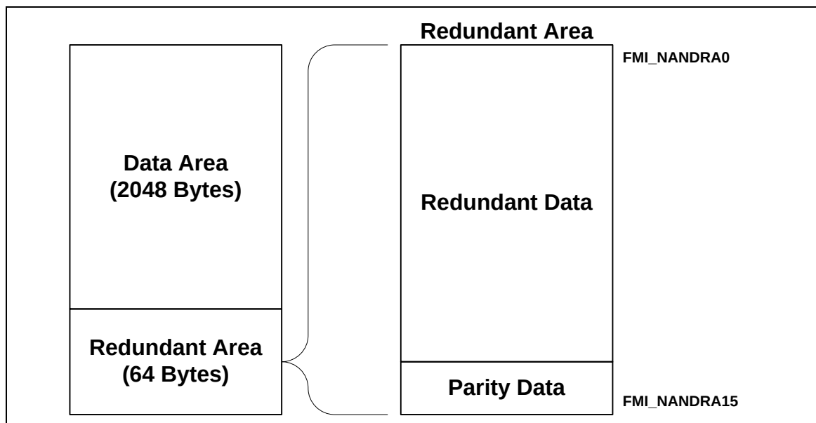
Figure 5.24-2 Data Arrangement for 2 kB Page Size NAND Flash
