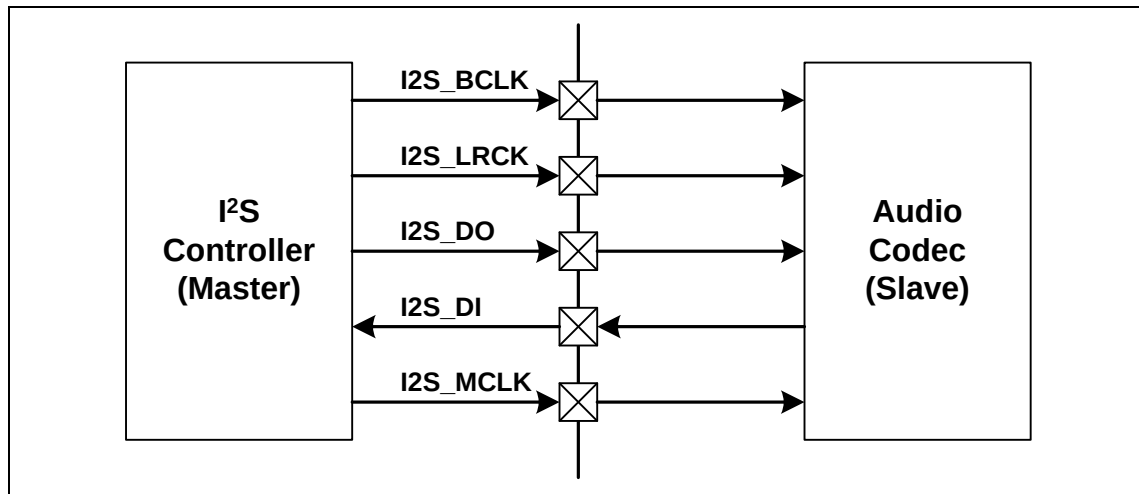
Figure 5.19-2 I 2 S Interface Signal of Master Mode
