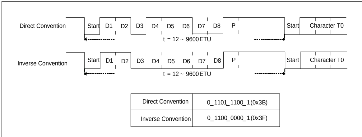
Figure 5.16-8 Initial Character TS
