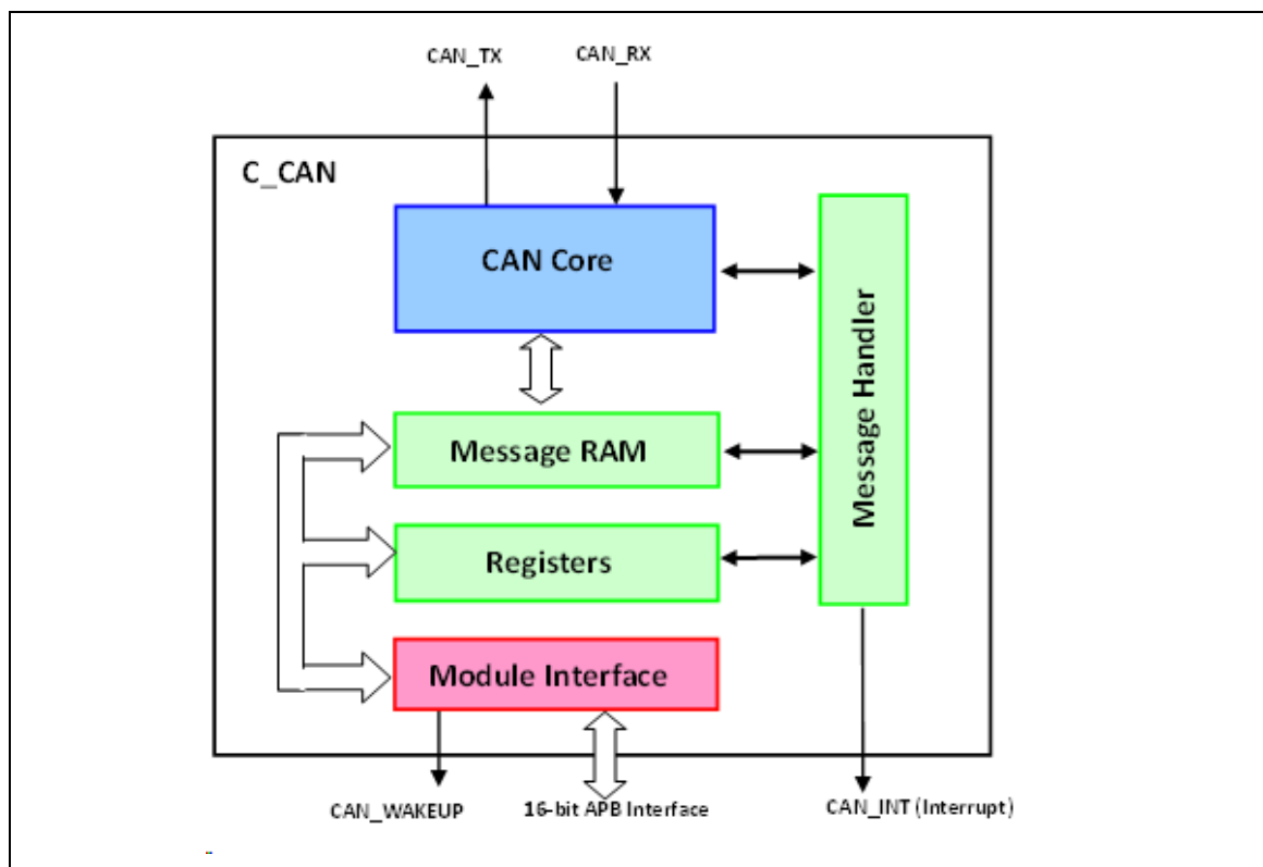
Figure 5.23-1 CAN Peripheral Block Diagram
