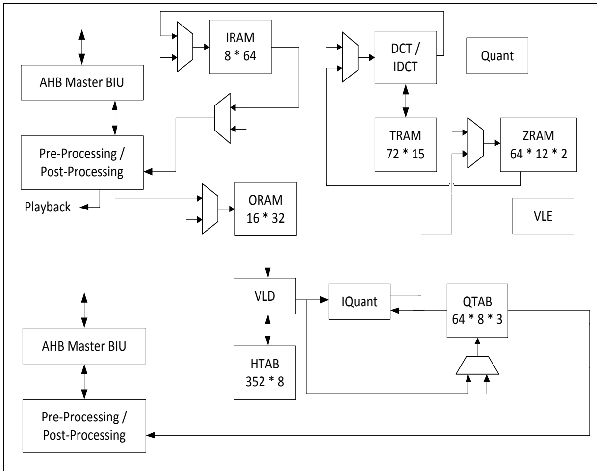
Figure 5.27-2 JPEG Codec block diagram (Decode)
