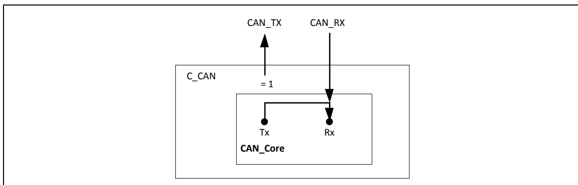
Figure 5.23-2 CAN Core in Silent Mode
