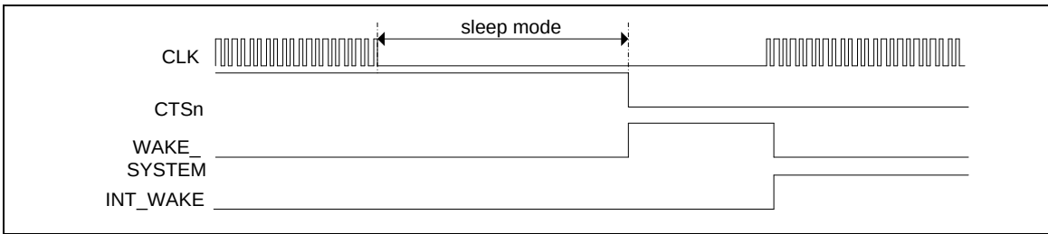
Figure 5.15-7 UART CTSn Wake-Up Case 2
