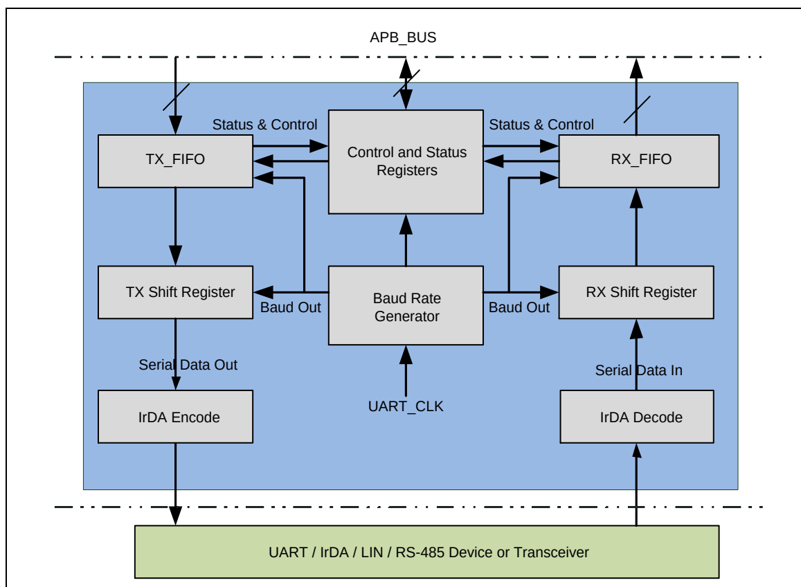
Figure 5.15-1 UART Block Diagram
