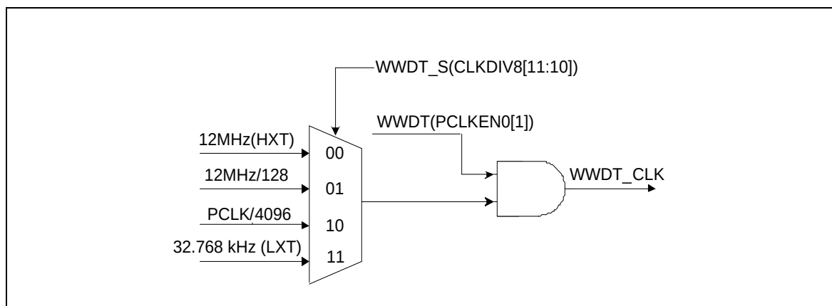
Figure 5.13-2 WWDT Clock Control
