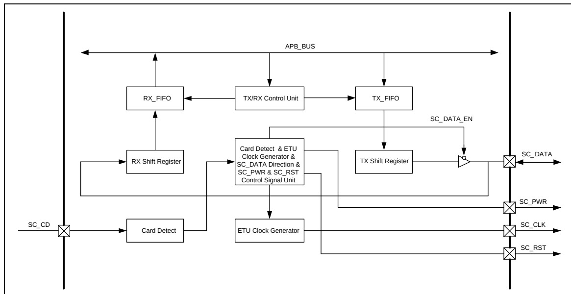
Figure 5.16-2 SC Controller Block Diagram
