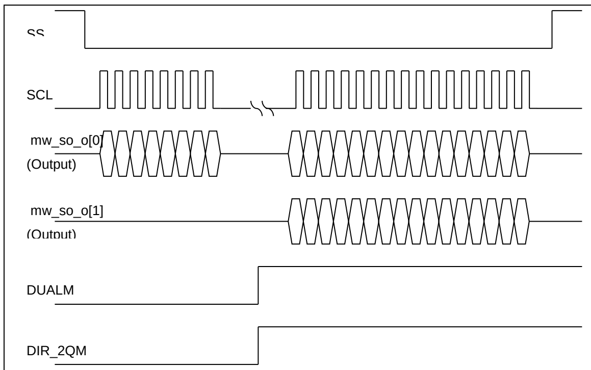
Figure 5.18-4 Dual-IO output Sequence
