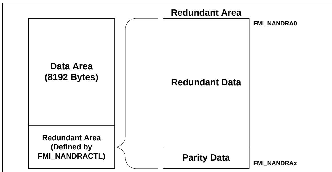
Figure 5.24-4 Data Arrangement for 8 kB Page Size NAND Flash
