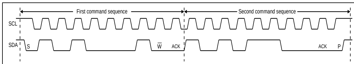
Figure 5.17-9 Write 1 byte of data to a slave
