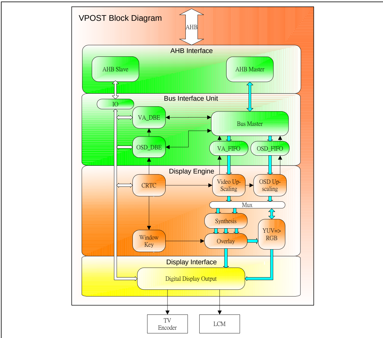
Figure 5.28-1 LCD Display Interface Controller Functional Block Diagram
