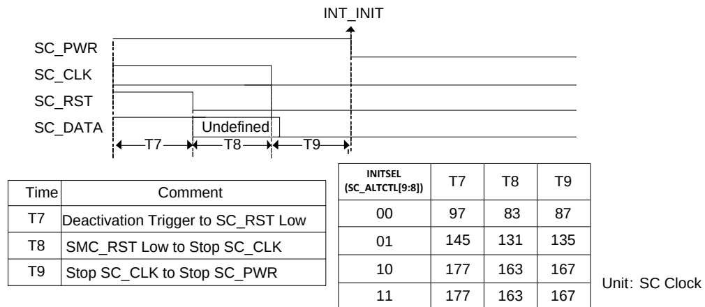
Figure 5.16-6 SC Deactivation Sequence
