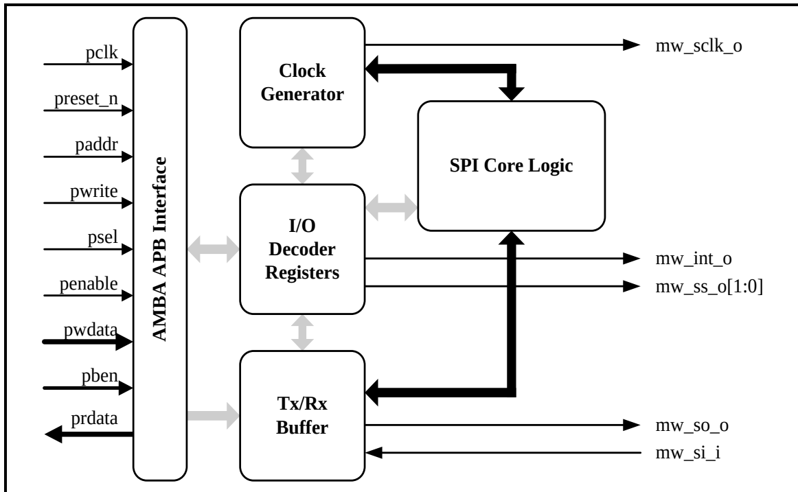
Figure 5.18-1 SPI Block Diagram
