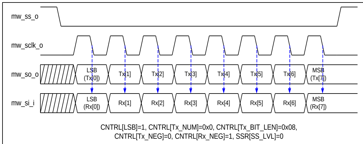
Figure 5.18-3 Alternate Phase SCLK Clock Timing
