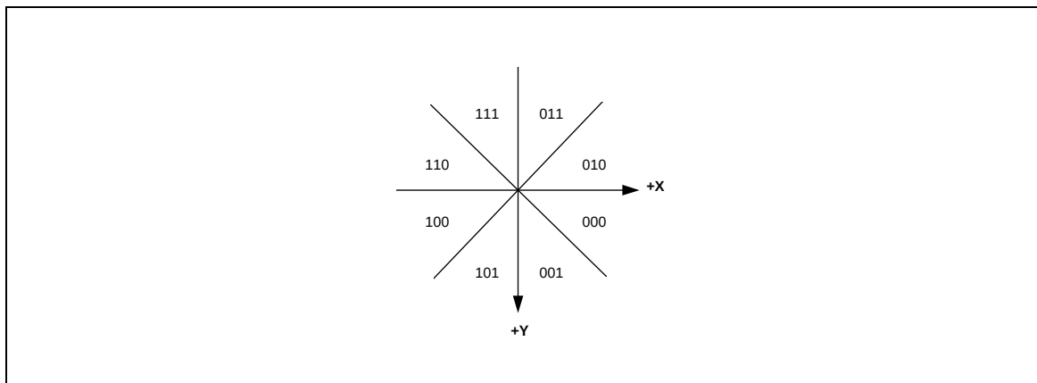
Figure 5.26-3 Bresenham Line Drawing Octant
