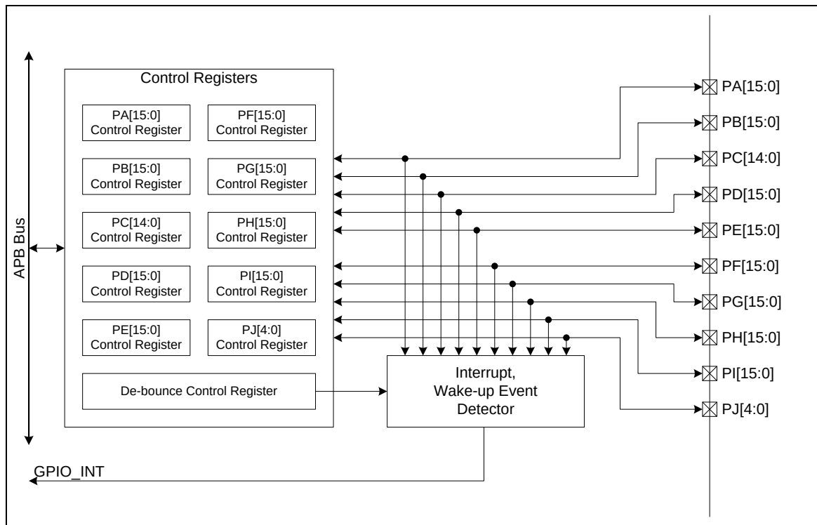
Figure 5.7-1 GPIO Block Diagram
