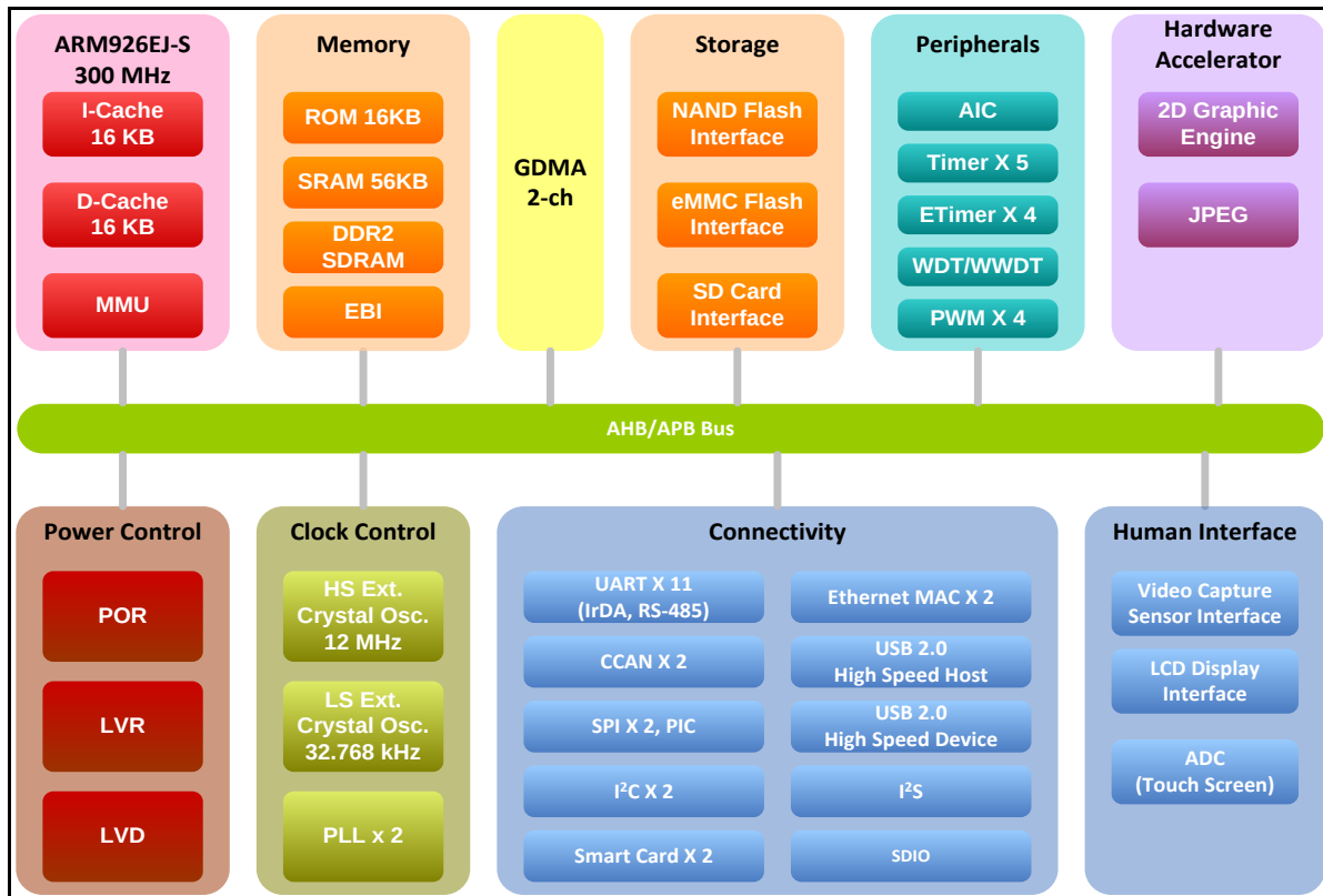
Figure 4.1-1 N9H30 Series Block Diagram
