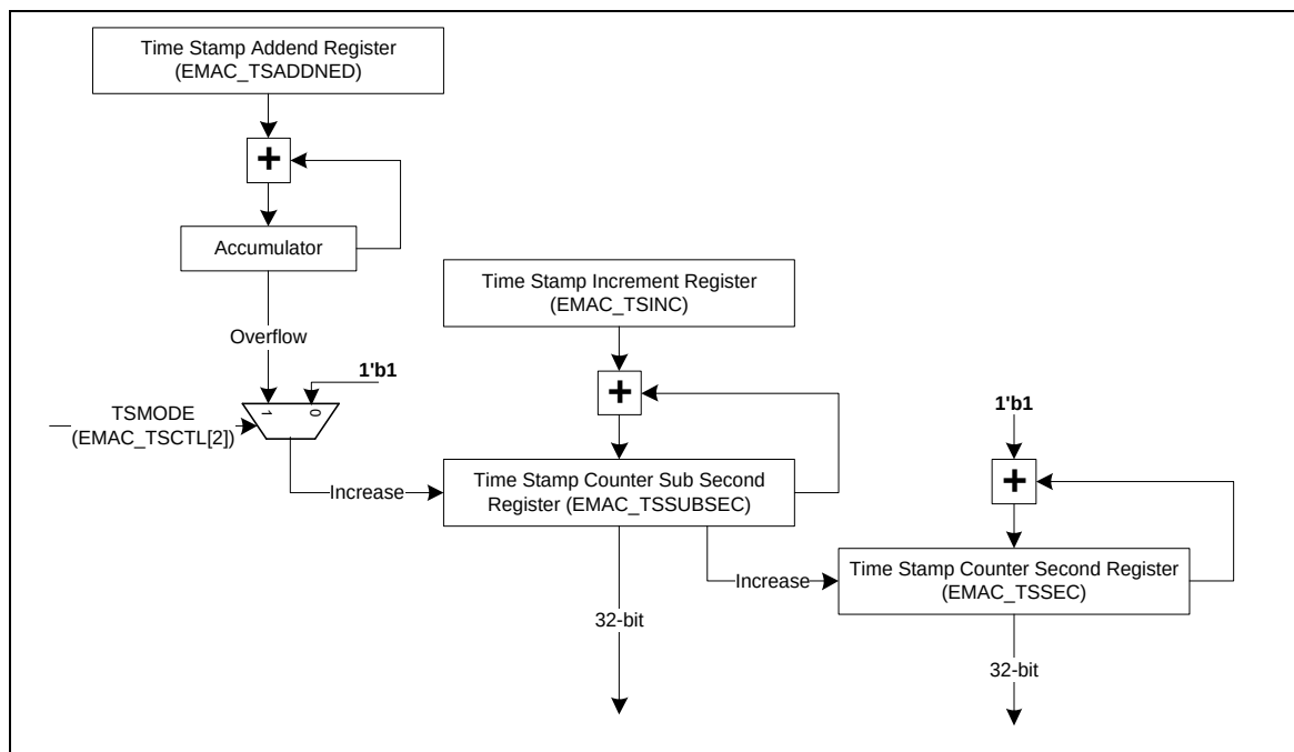
Figure 5.20-3 64-bit Reference Timing Counter
