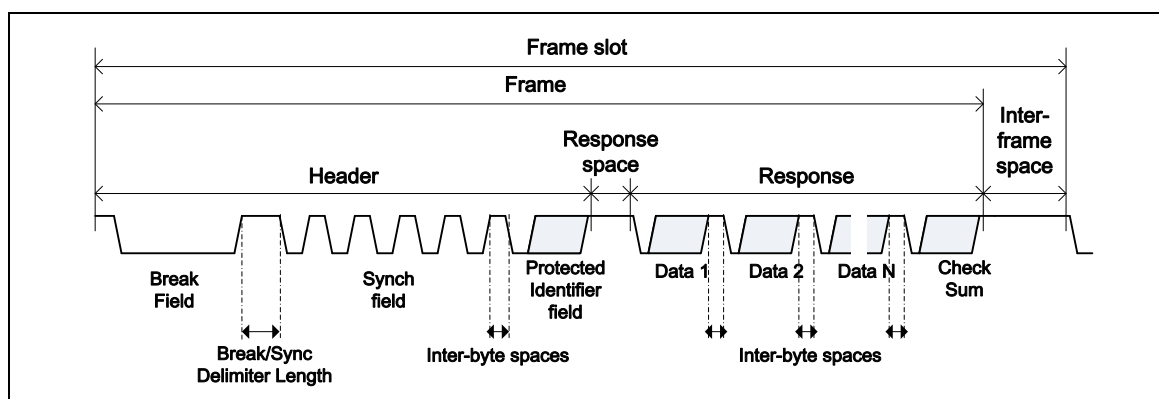
Figure 5.15-11 LIN Frame Structure
