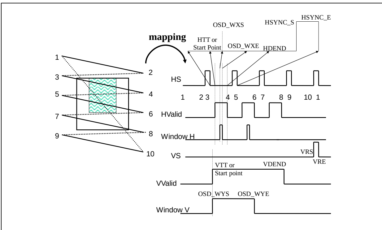
Figure 5.28-2 Display and Overlay Control Timing
