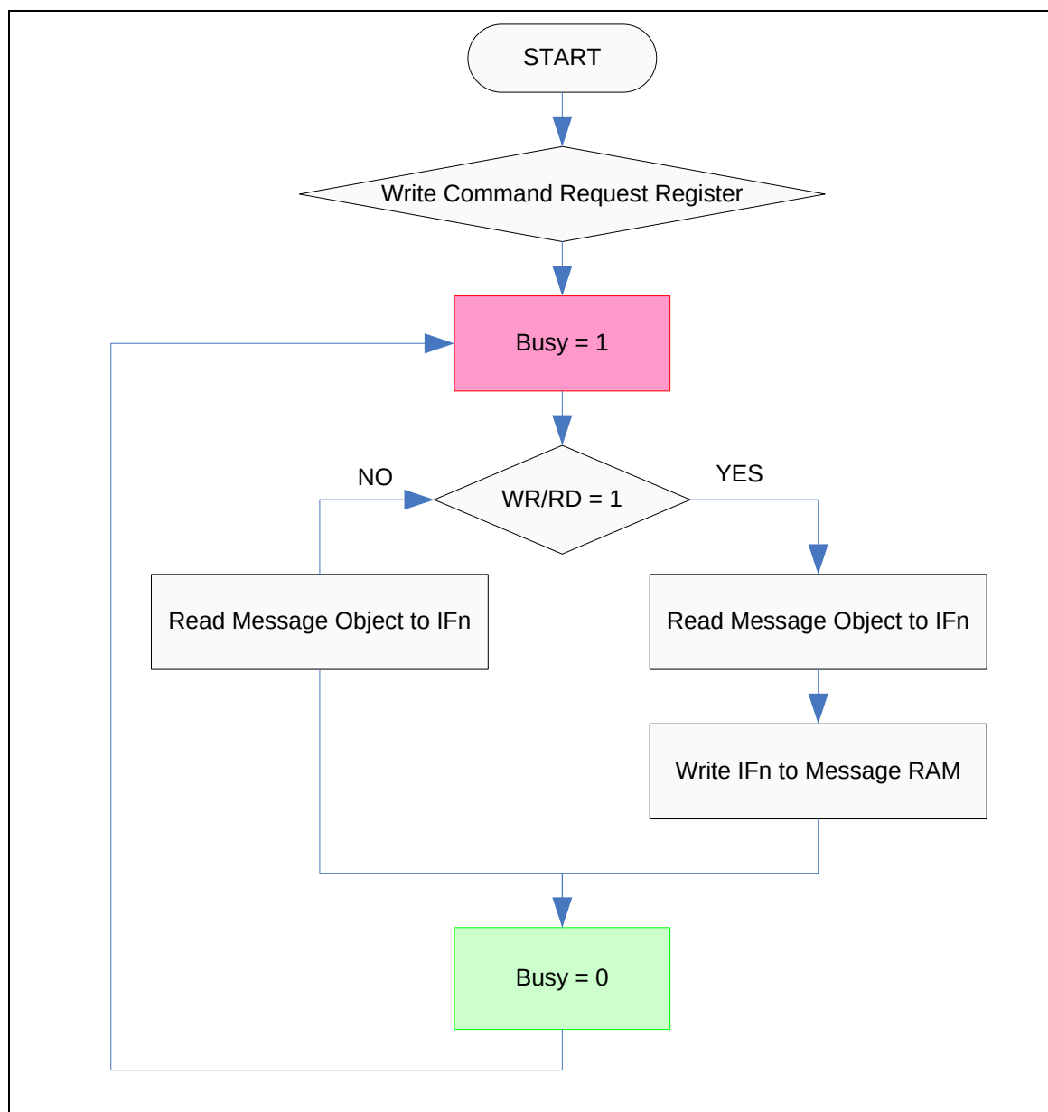
Figure 5.23-5 Data transfer between IFn Registers and Message
