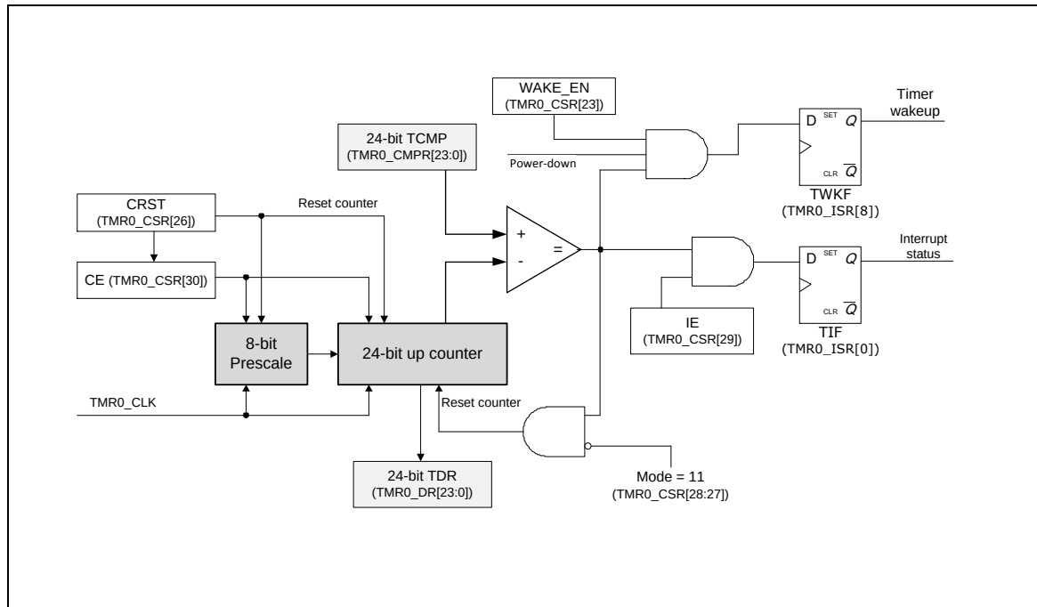
Figure 5.9-1 Timer Controller Block Diagram
