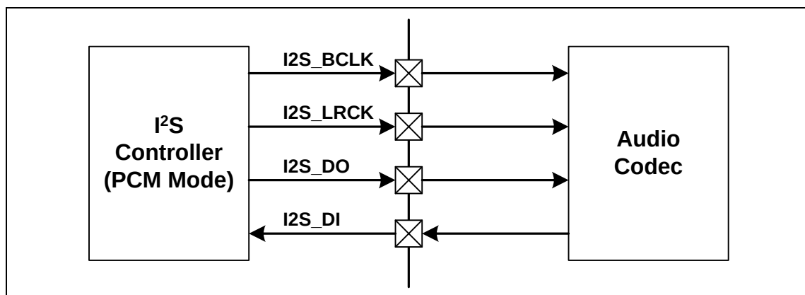
Figure 5.19-5 PCM Mode Signal Interface
