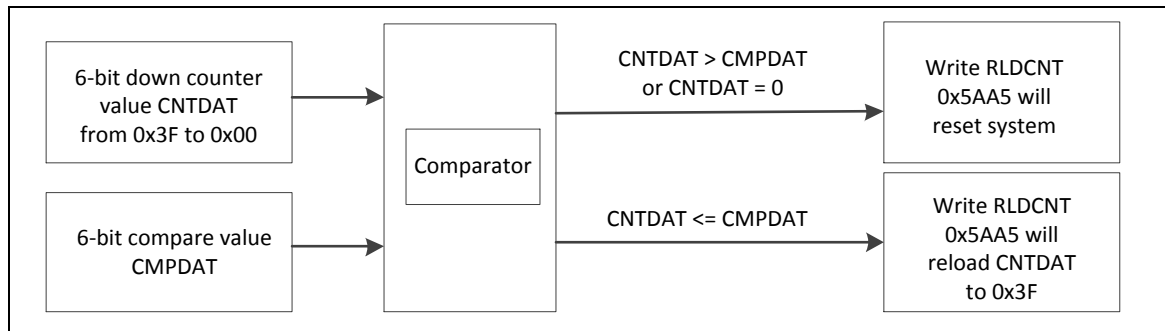
Figure 5.13-3 WWDT Reset and Reload Behavior
