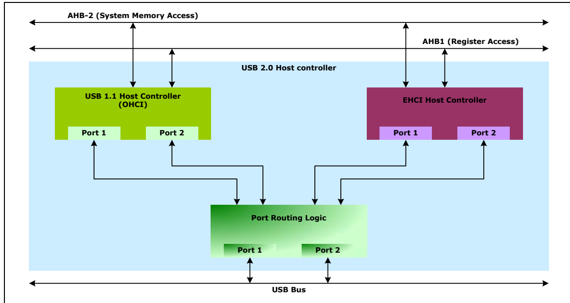
Figure 5.22-1 USB Host Controller Block Diagram
