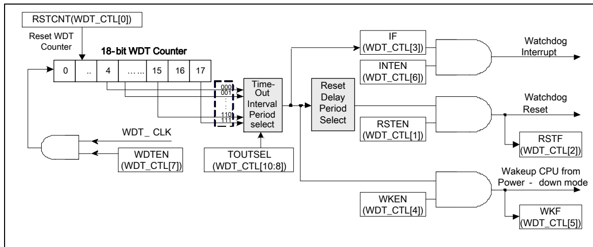
Figure 5.12-1 Watchdog Timer Block Diagram
