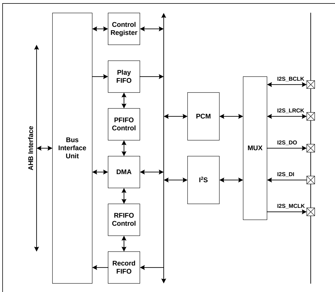
Figure 5.19-1 I 2 S Controller Block Diagram
