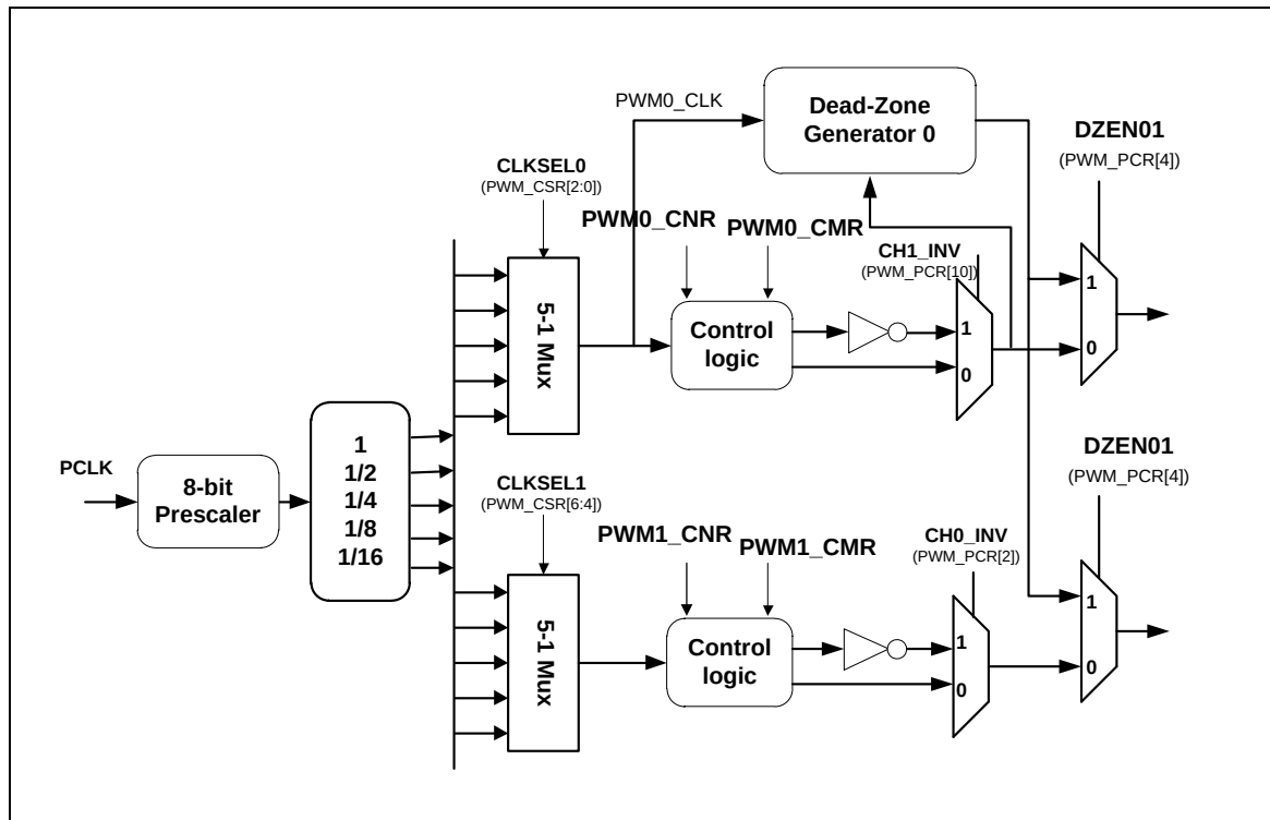
Figure 5.11-1 Two channels of PWM in one pair
