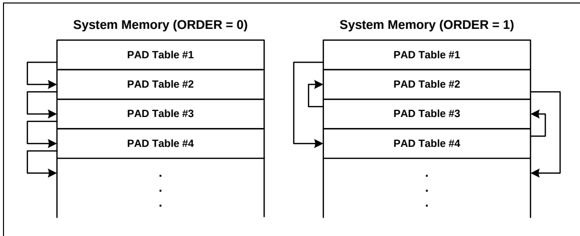
Figure 5.24-6 PAD (Physical Address Descriptor) Table Fetch Modes
