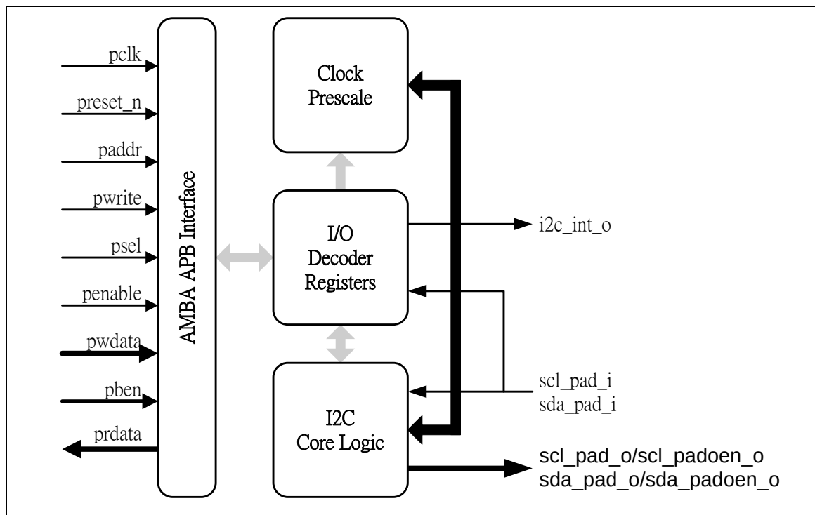
Figure 5.17-1 I 2 C Block Diagram
