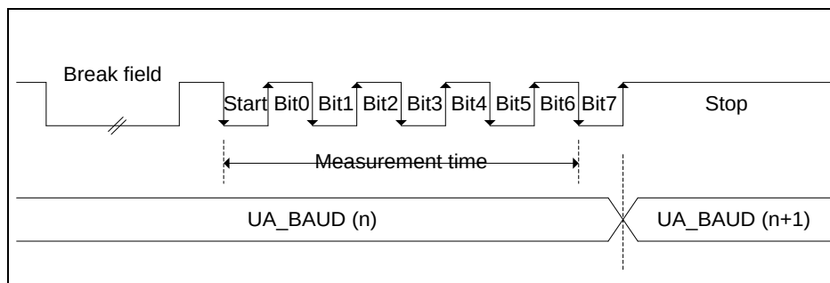
Figure 5.15-14 LIN Sync Field Measurement
