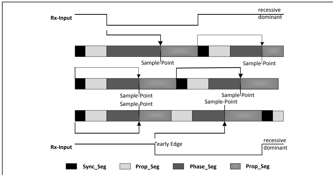
Figure 5.23-9 Synchronization on “late” and “early” Edges
