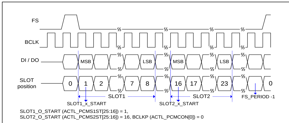
Figure 5.19-6 PCM Mode Interface Waveform
