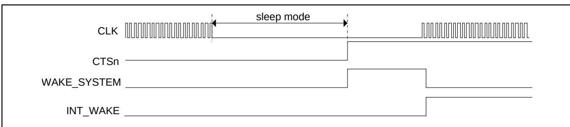
Figure 5.15-6 UART CTSn Wake-Up Case 1
