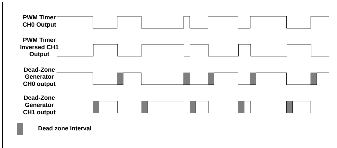
Figure 5.11-5 Paired PWM Output with Dead Zone Generation Operation
