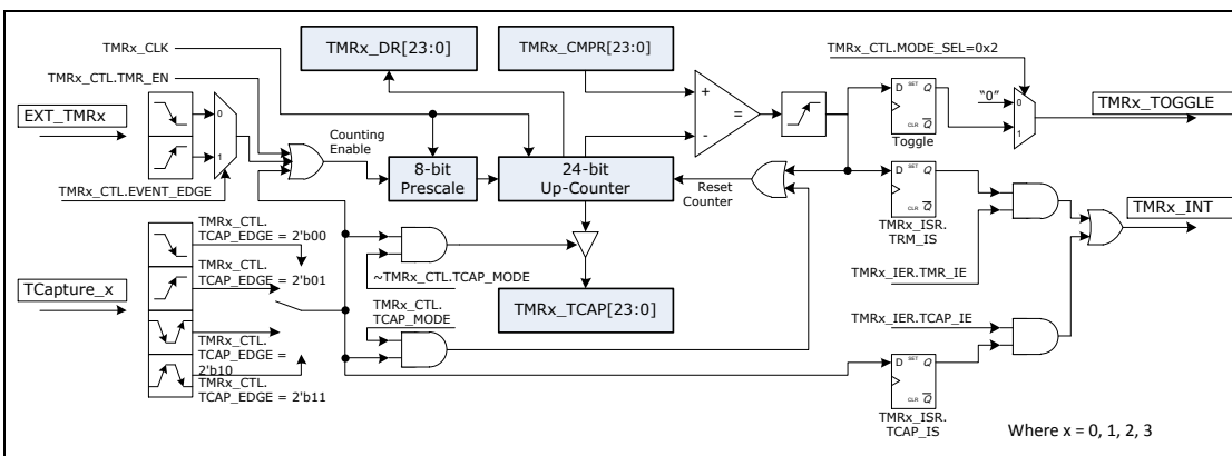
Figure 5.10-1 Enhance Timer Controller Block Diagram
