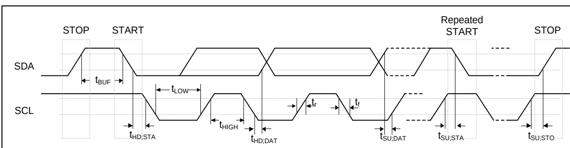
Figure 5.17-2 I 2 C Bus Timing
