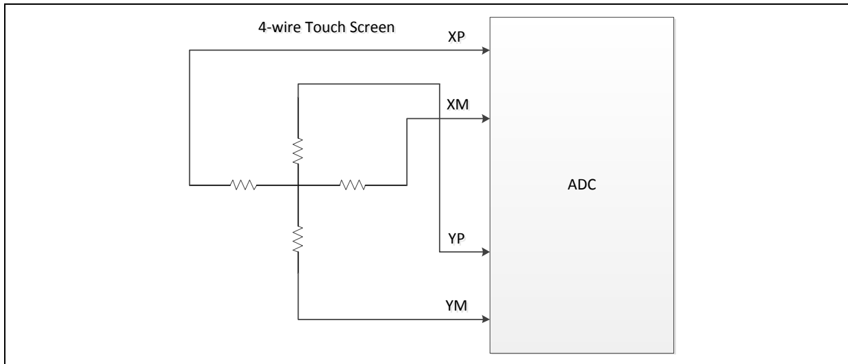
Figure 5.30-7 4-wire Touch Screen Connection Diagram
