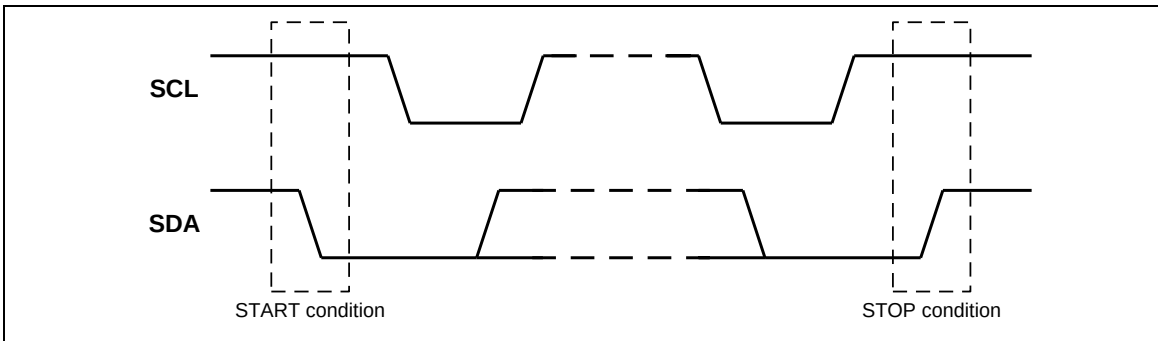
Figure 5.17-4 START and STOP conditions
