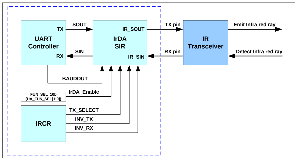
Figure 5.15-8 IrDA Block Diagram
