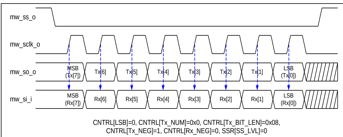
Figure 5.18-2 Normal SPI Timing
