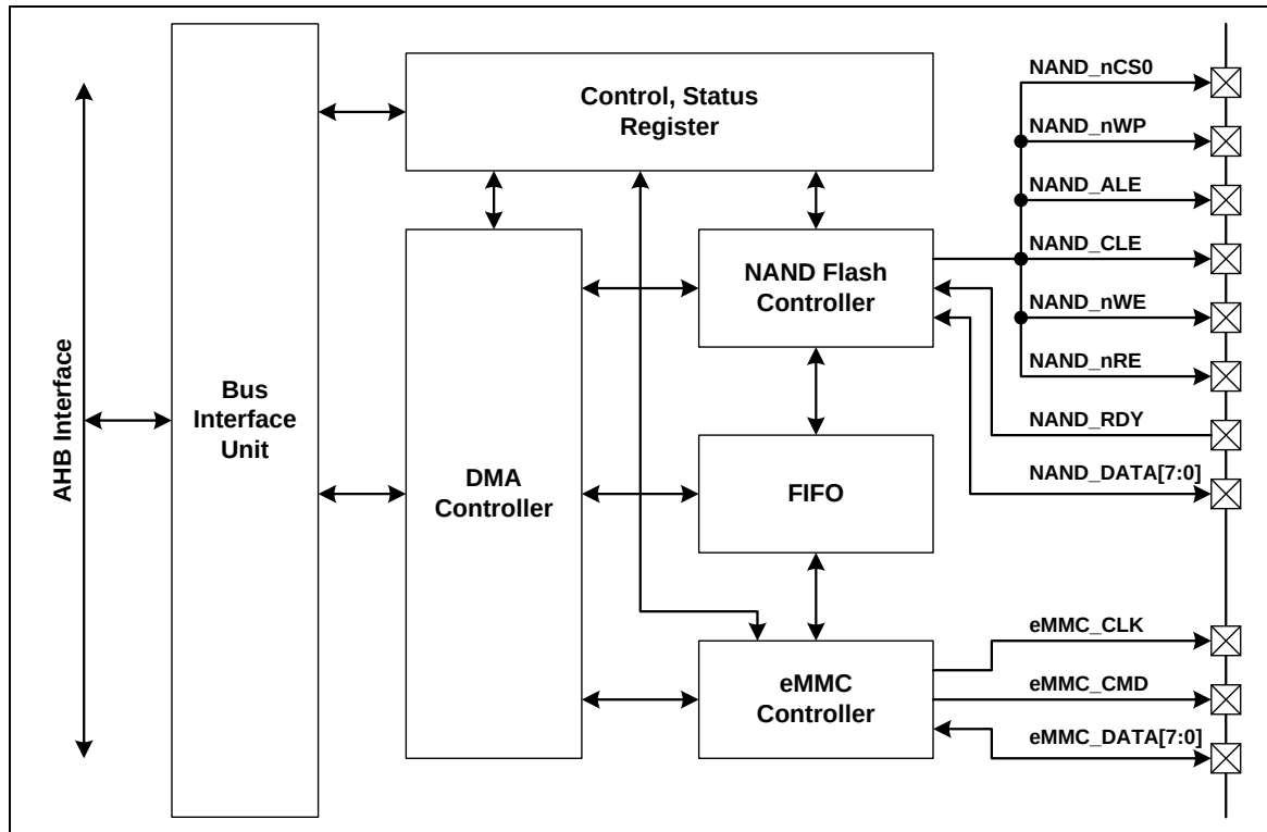
Figure 5.24-1 FMI Block Diagram
