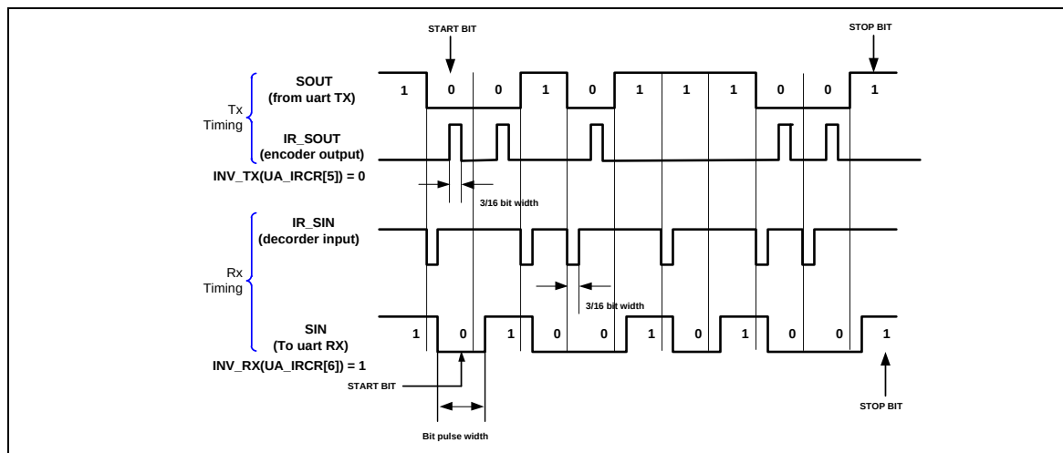
Figure 5.15-9 IrDA TX/RX Timing Diagram
