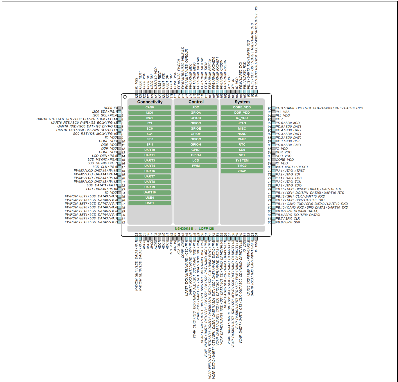
Figure 3.3-1 N9H30Kxxl Series LQFP 128-pin Pin Diagram
