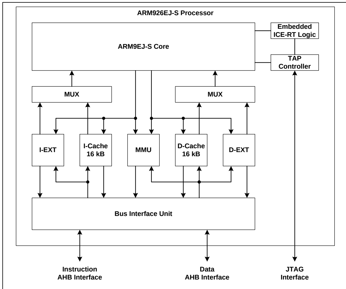
Figure 5.1-1 ARM926EJ-S Block Diagram
