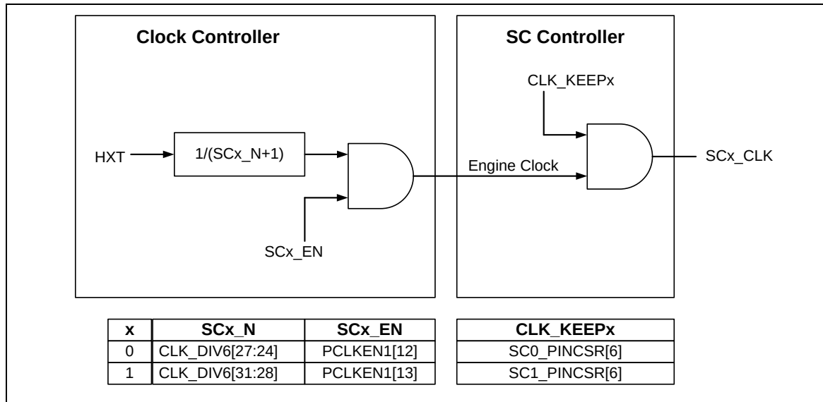
Figure 5.16-1 SC Clock Control Diagram (4-bit Prescale Counter in Clock Controller)
