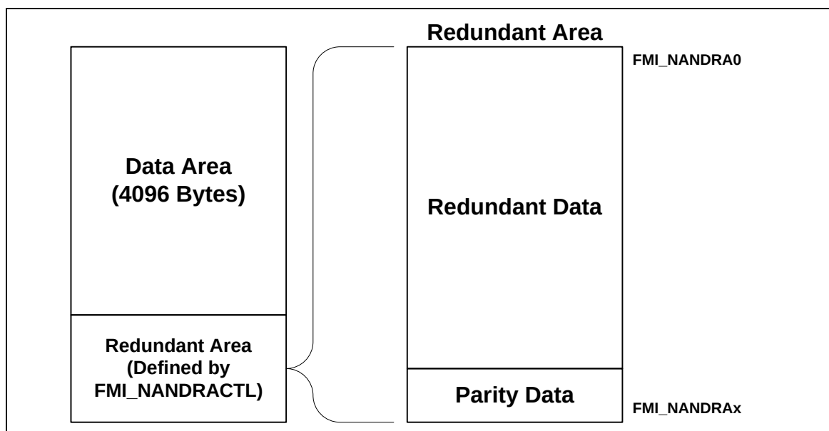
Figure 5.24-3 Data Arrangement for 4 kB Page Size NAND Flash
