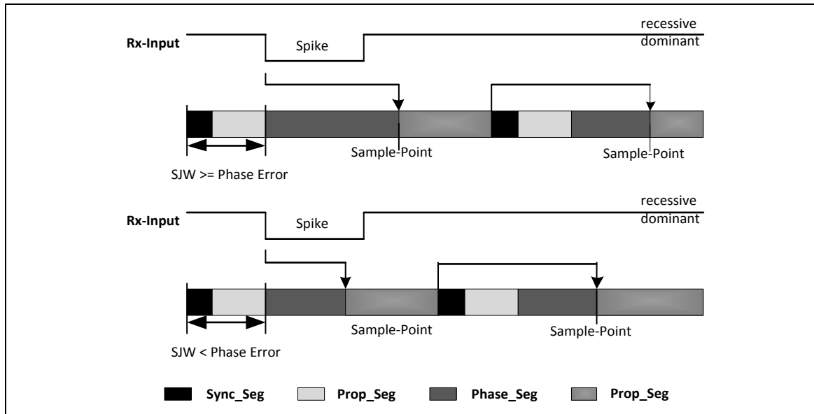
Figure 5.23-10 Filtering of Short Dominant Spikes
