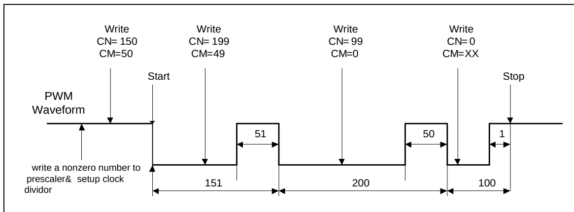
Figure 5.11-3 PWM Double Buffer Illustration
