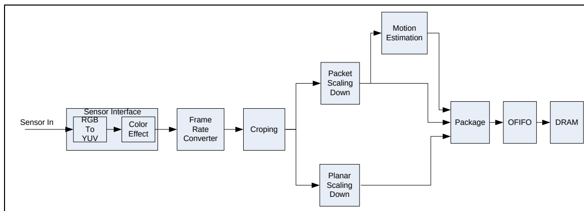
Figure 5.29-1 Image Capture Functional Block Diagram
