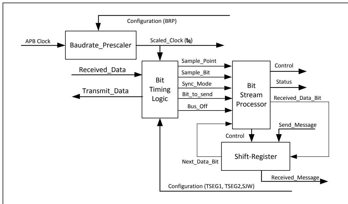
Figure 5.23-11 Structure of the CAN Core's CAN Protocol Controller
