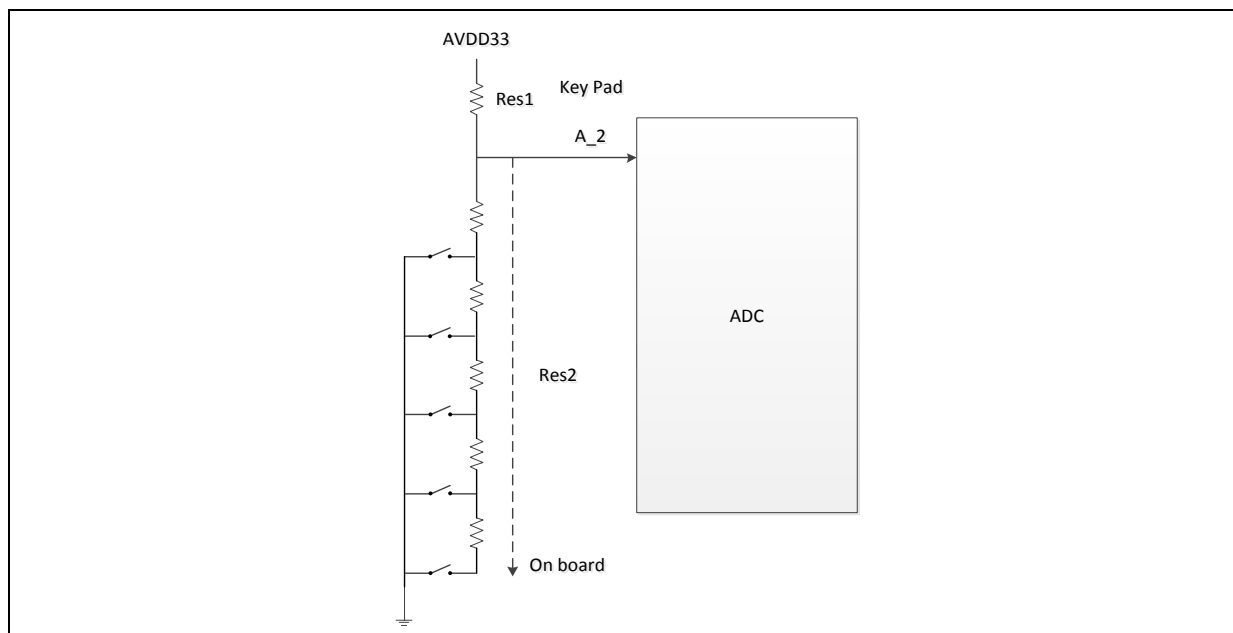
Figure 5.30-6 Key Pad Detection Diagram
