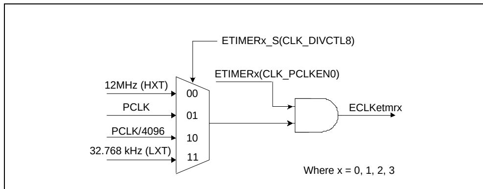
Figure 5.10-2 Enhance Timer Clock Controller Diagram
