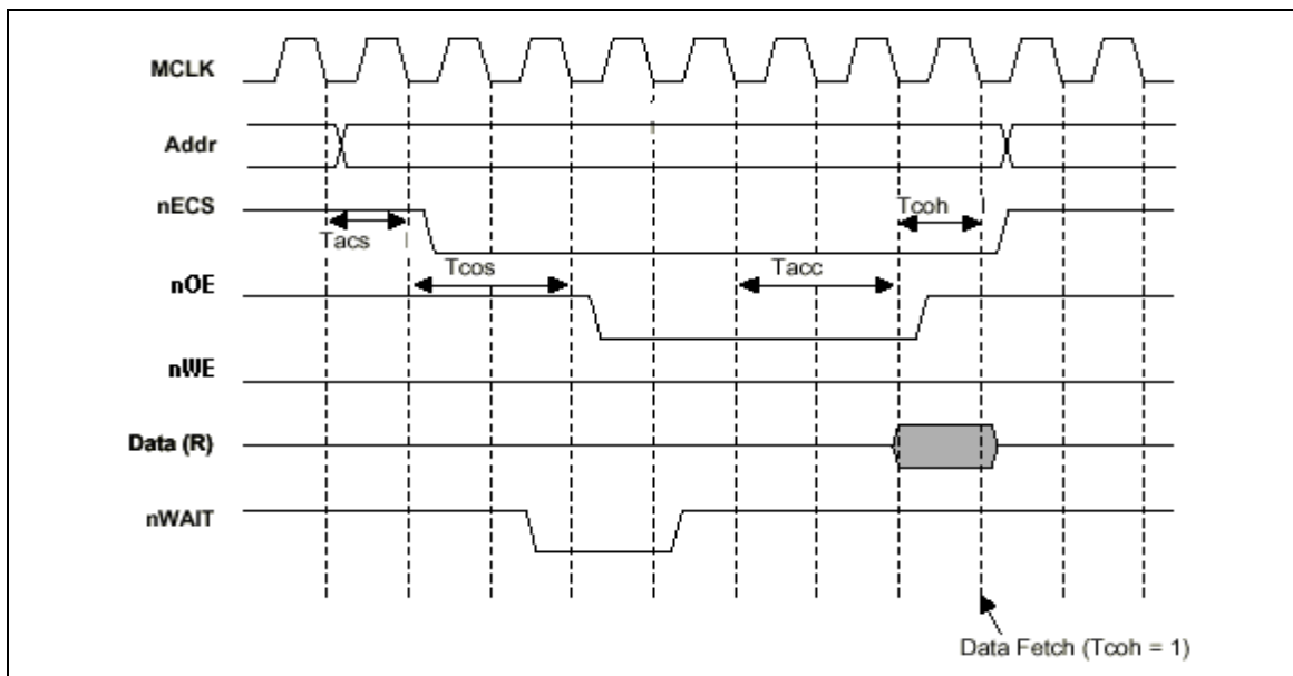
Figure 5.6-3 External I/O Read operation timing
