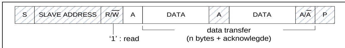
Figure 5.17-8 Master Reads Data from Slave
