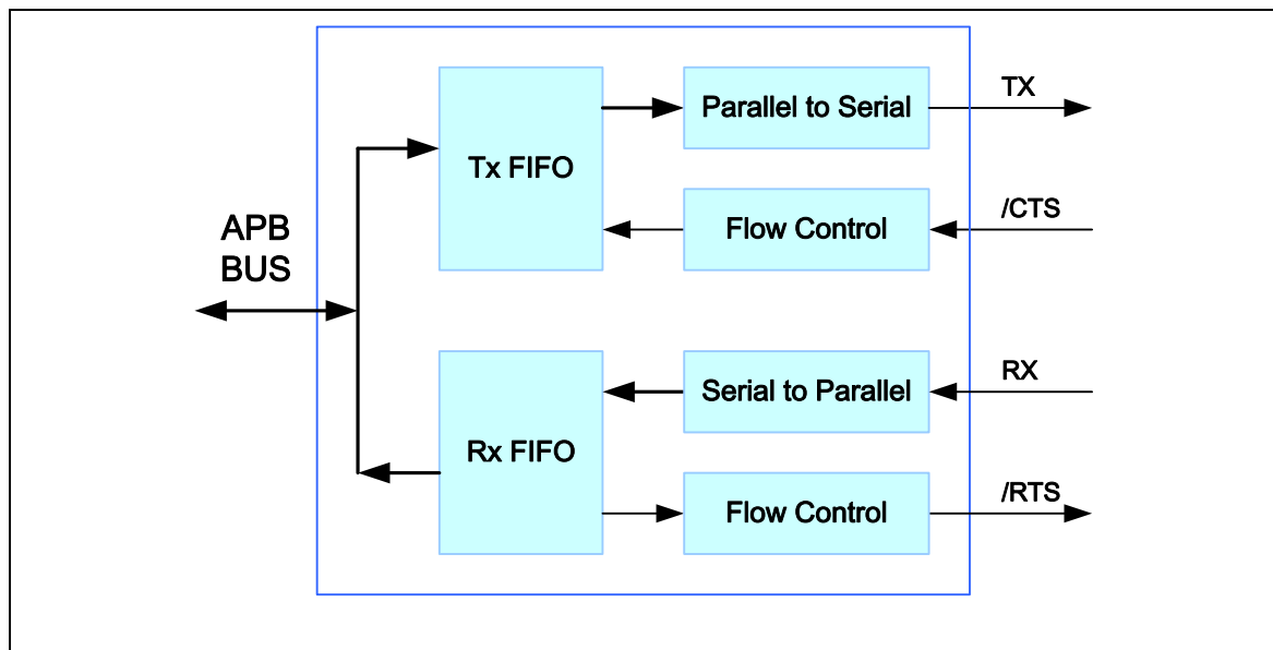
Figure 5.15-2 Auto Flow Control Block Diagram
