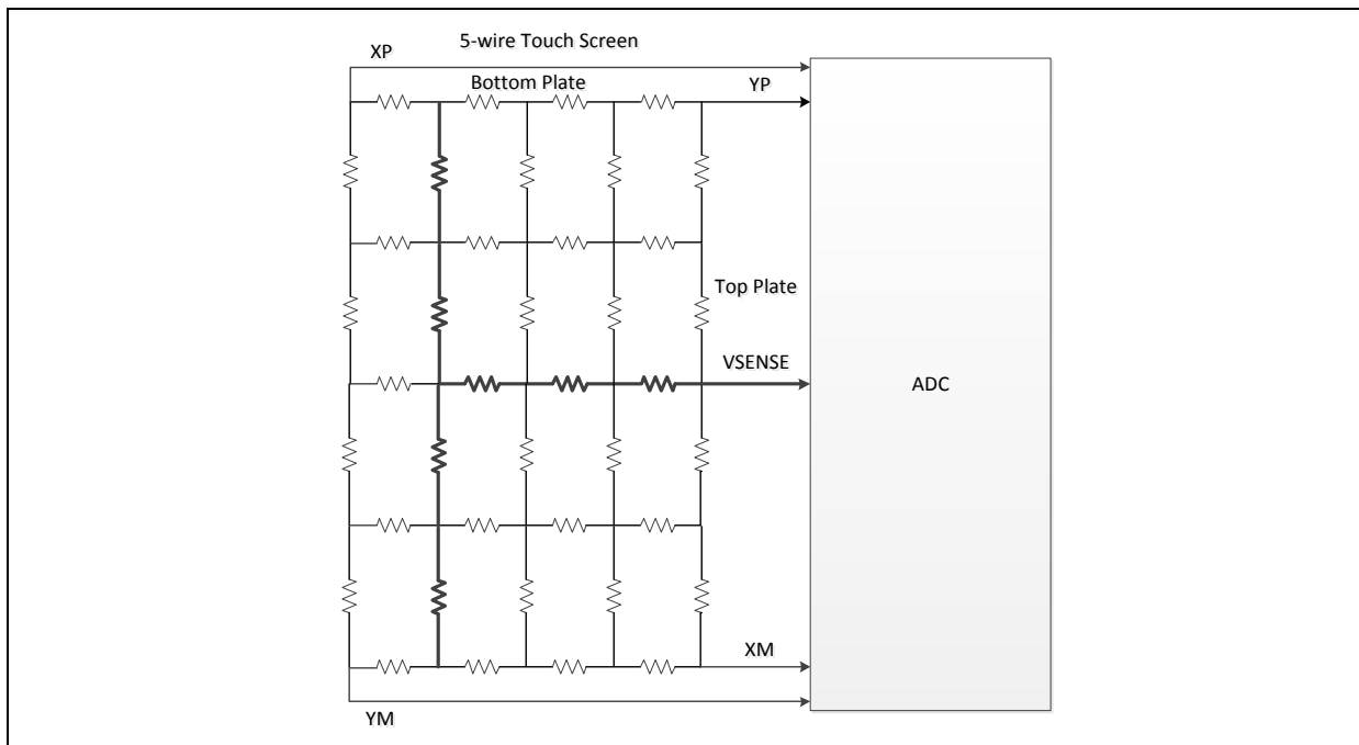
Figure 5.30-8 5-wire Touch Screen Connection Diagram
