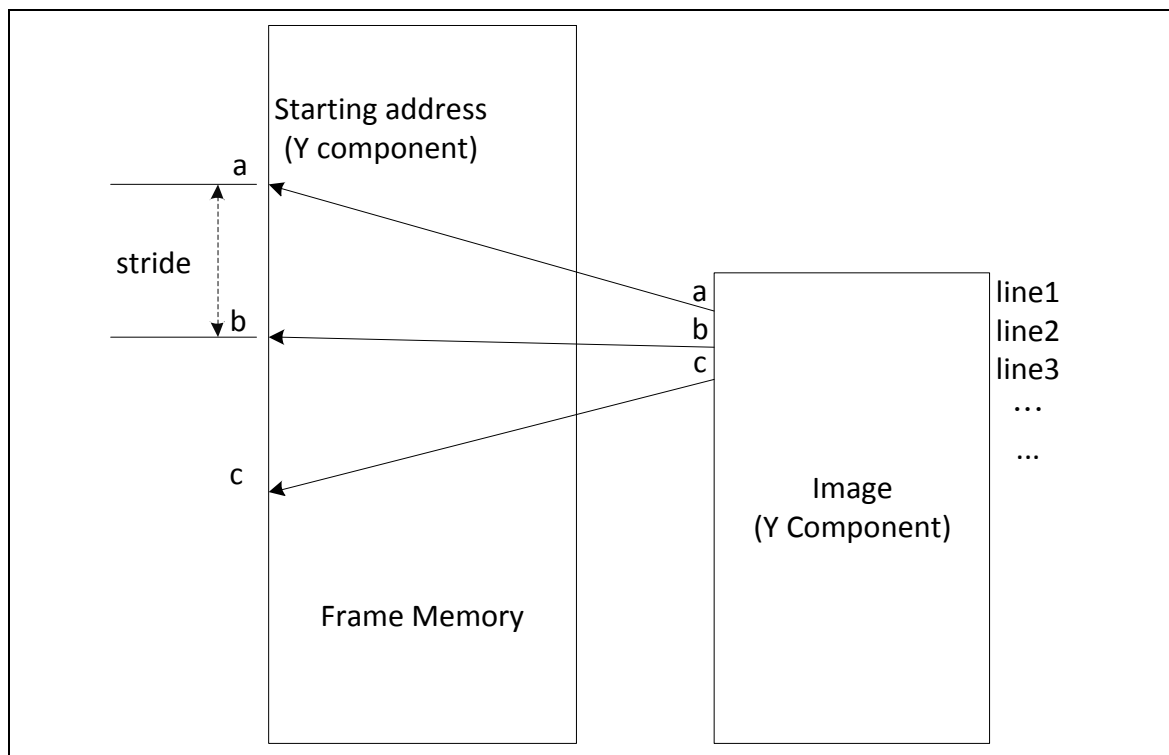
Figure 5.27-3 Image starting address and stride
