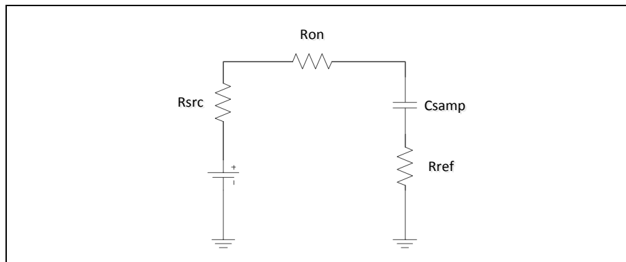
Figure 5.30-3 Simplified Sampling Diagram
