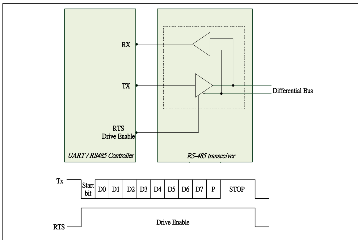
Figure 5.15-10 RS-485 Frame Structure
