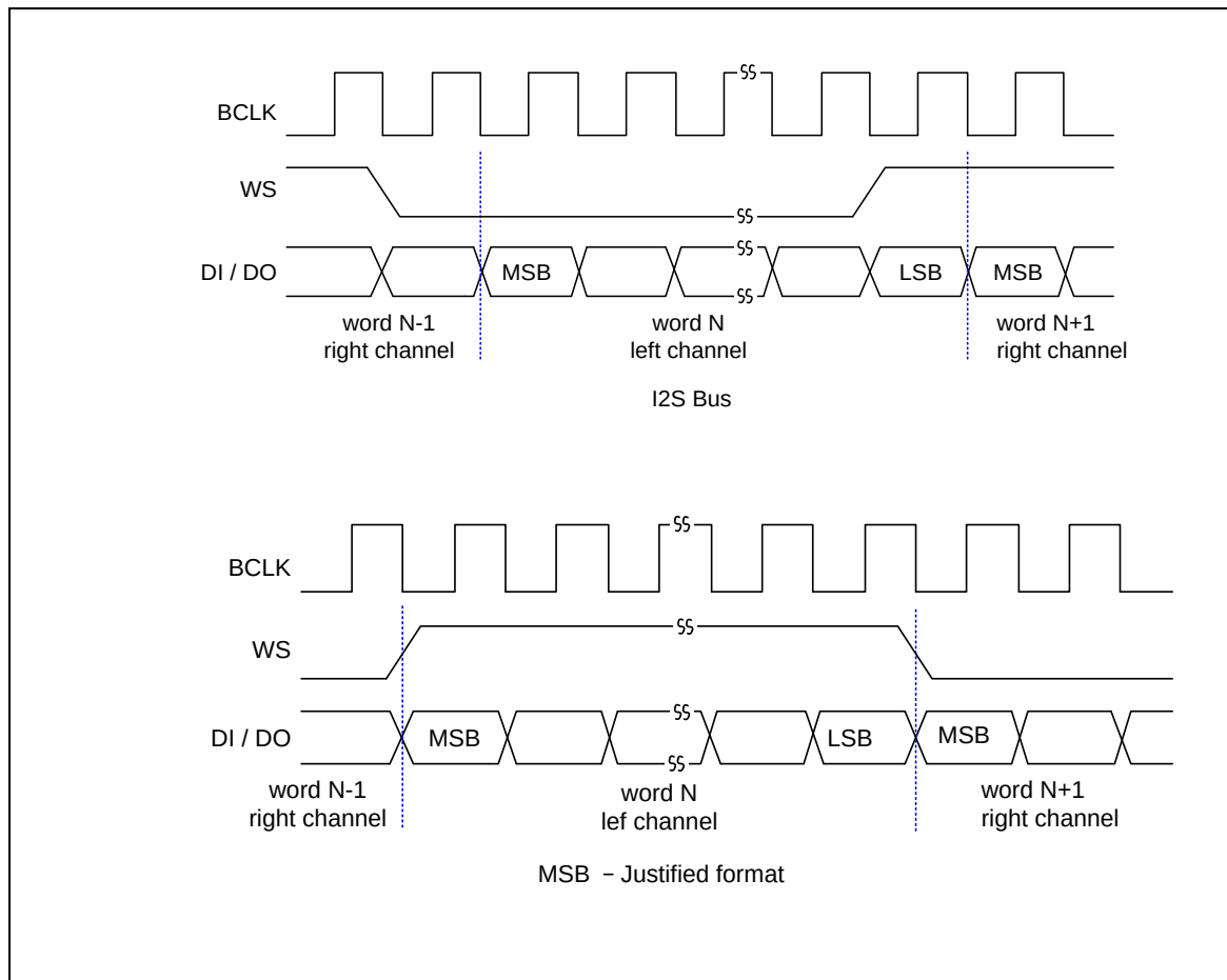
Figure 5.19-4 I 2 S MSB-Justified Format
