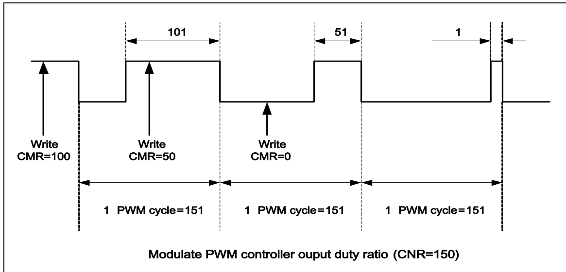
Figure 5.11-4 PWM Controller Output Duty Ratio
