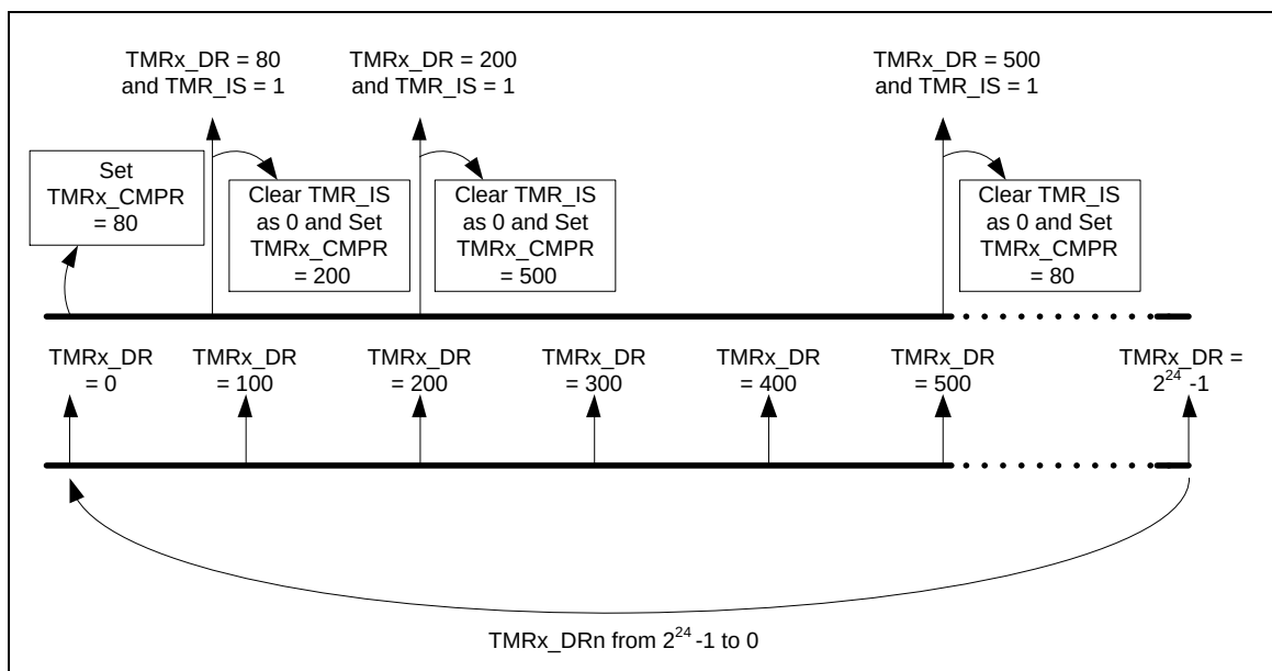
Figure 5.10-3 Timer Clock Controller Diagram
