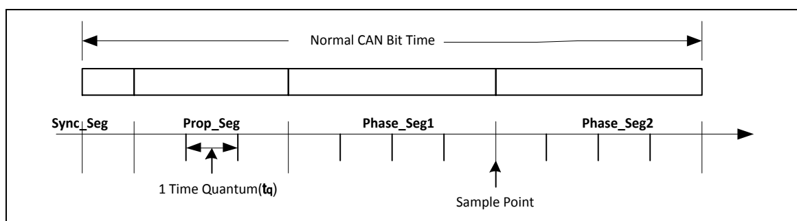
Figure 5.23-7 Bit Timing
