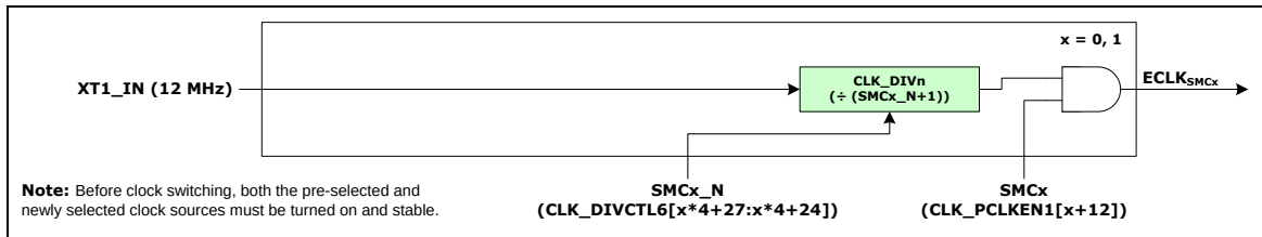
Figure 5.3-11 Smart Card Host Controller Clock Divider Block Diagram
