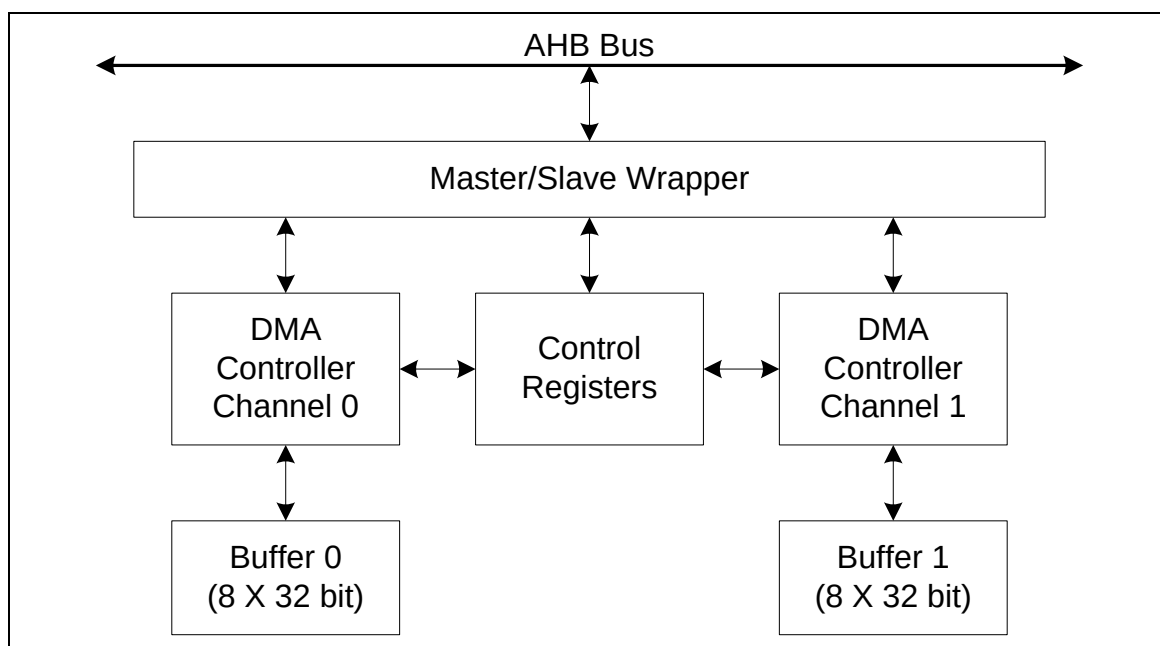
Figure 5.8-1 GDMA Block Diagram
