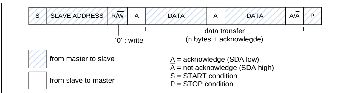
Figure 5.17-7 Master Transmits Data to Slave
