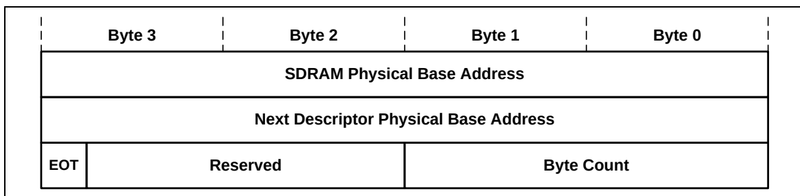
Figure 5.25-1 PAD (Physical Address Descriptor) Table Format
