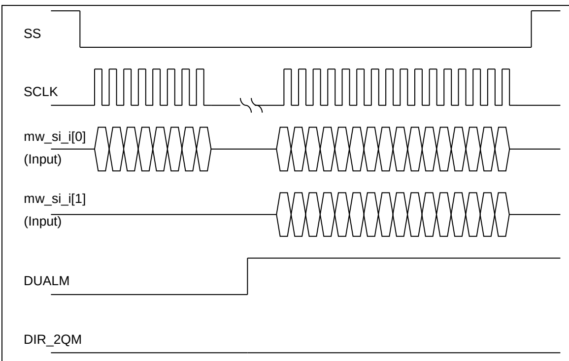
Figure 5.18-5 Dual-IO Input Sequence
