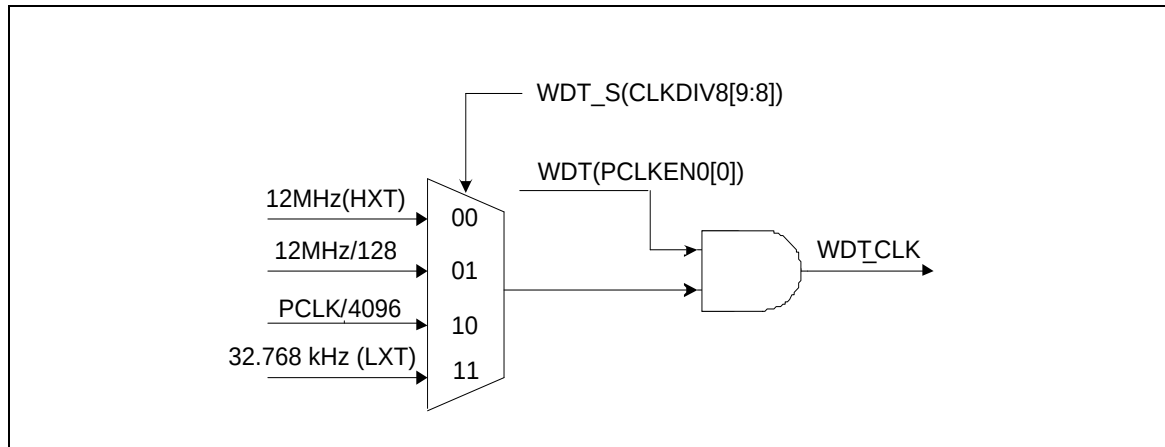
Figure 5.12-2 Watchdog Timer Clock Control
