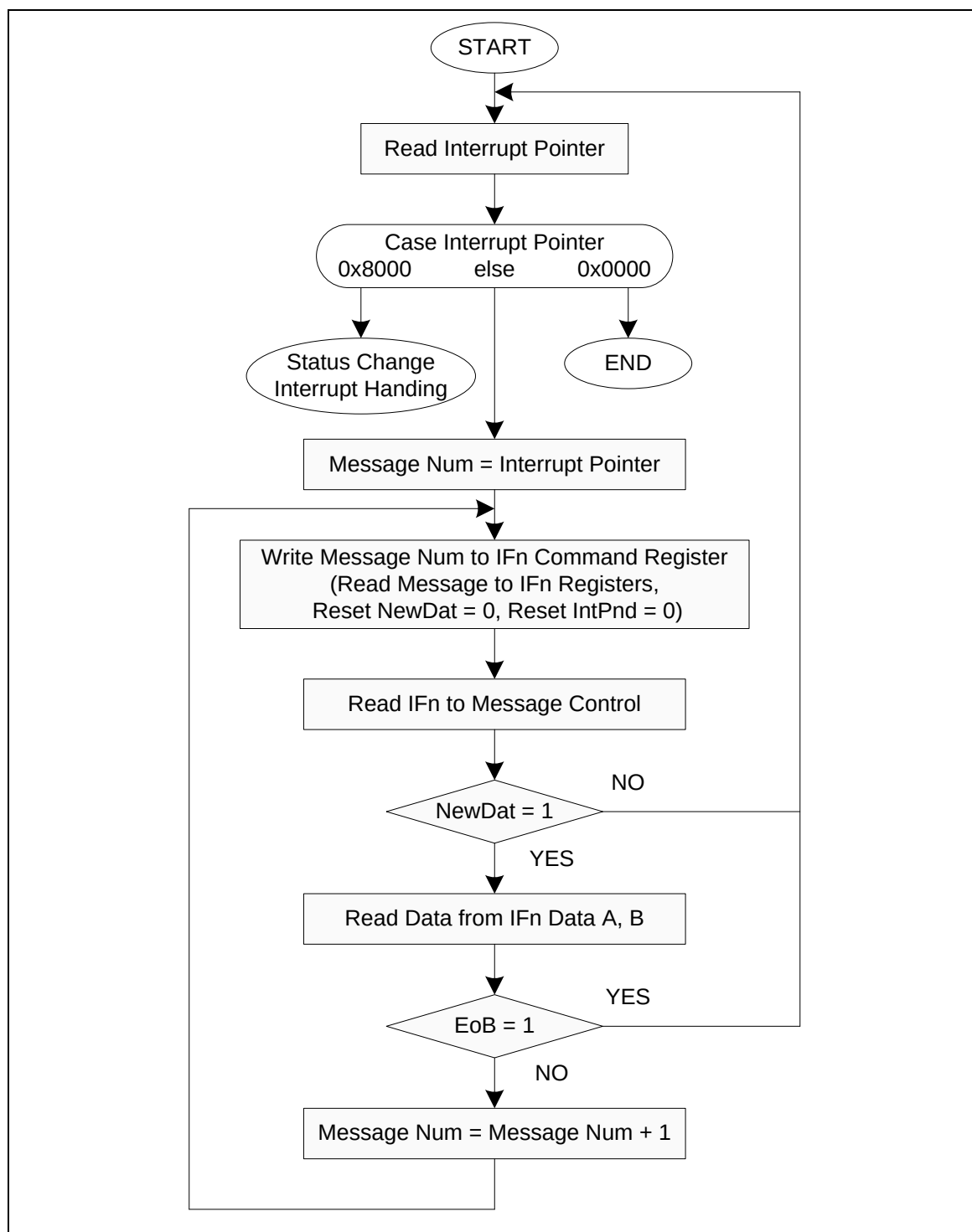
Figure 5.23-6 Application Software Handling of a FIFO Buffer
