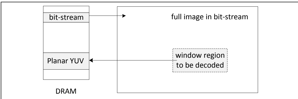
Figure 5.27-6 Specified window decode mode
