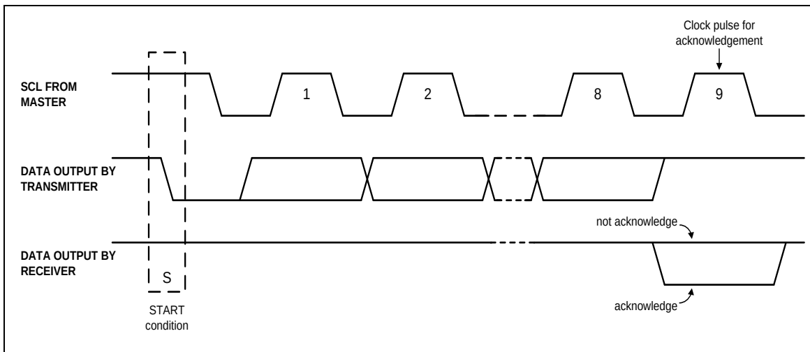
Figure 5.17-6 Acknowledge on the I 2 C-bus
