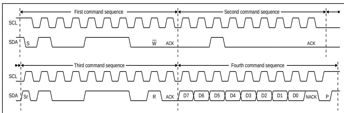
Figure 5.17-10 Read a byte of data
