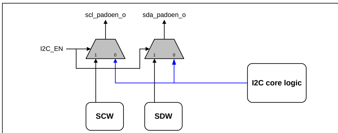
Figure 5.17-11 Implementation of Software I 2 C
