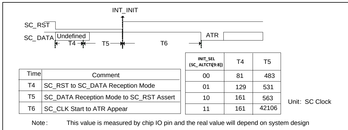
Figure 5.16-5 SC Warm Reset Sequence
