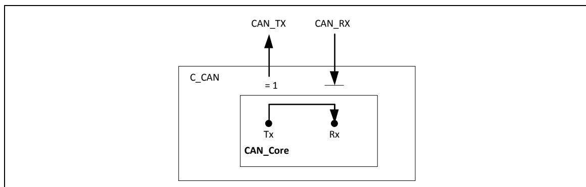
Figure 5.23-4 CAN Core in Loop Back Mode Combined with Silent Mode
