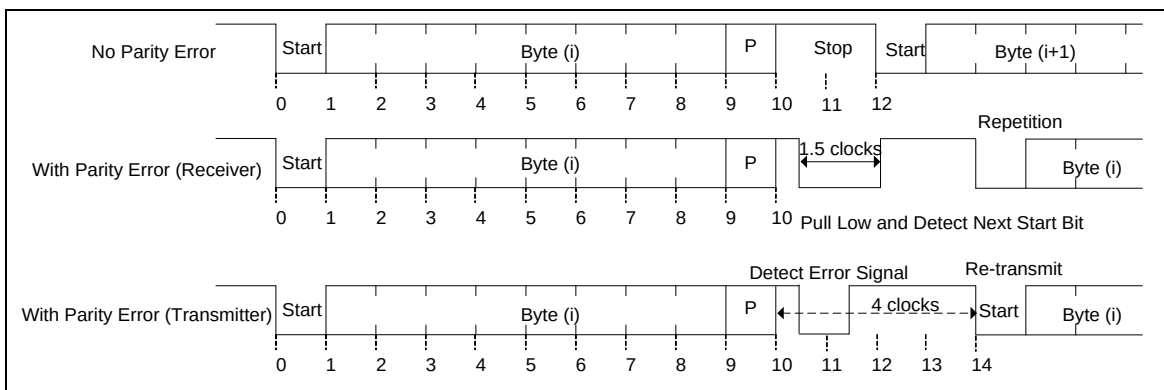
Figure 5.16-9 SC Error Signal
