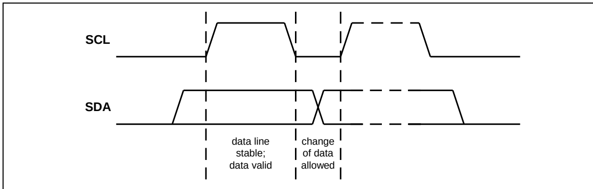
Figure 5.17-5 Bit transfer on the I 2 C-bus
