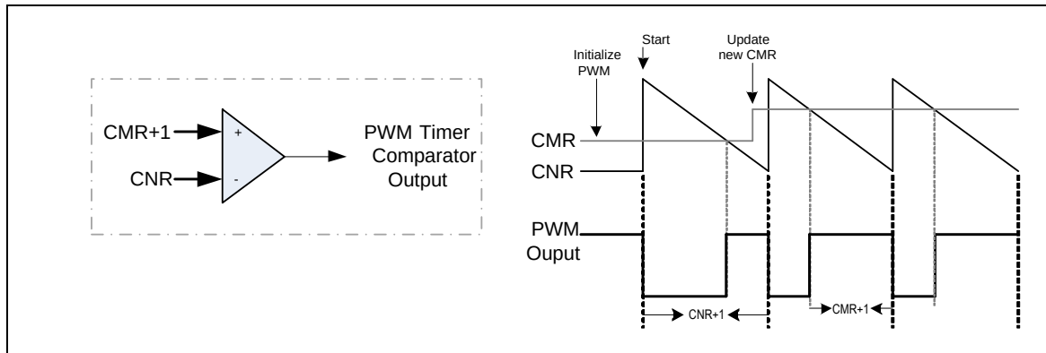
Figure 5.11-2 Legend of Internal Comparator Output of PWM-Timer
