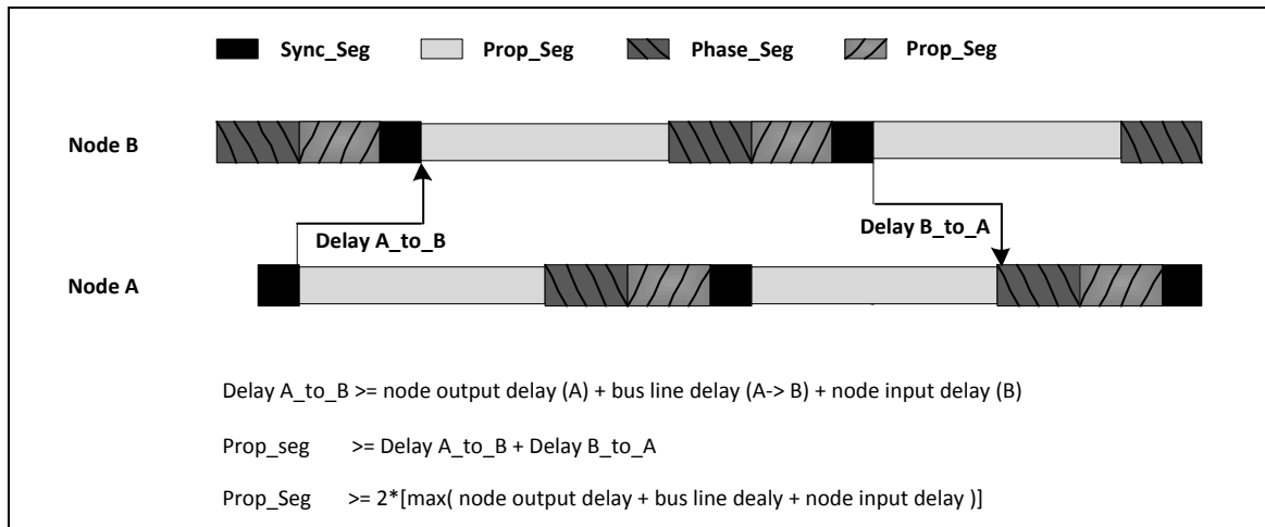
Figure 5.23-8 Propagation Time Segment
