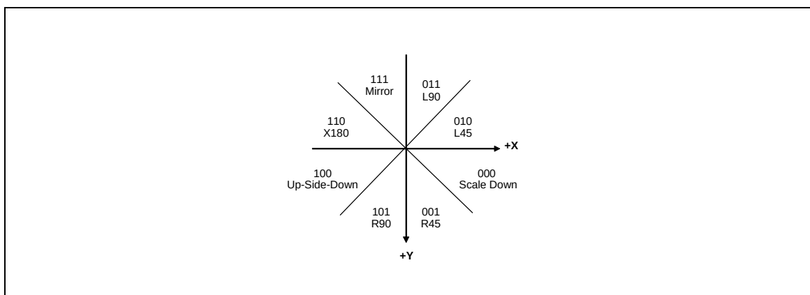
Figure 5.26-4 Rotation Operation Octant
