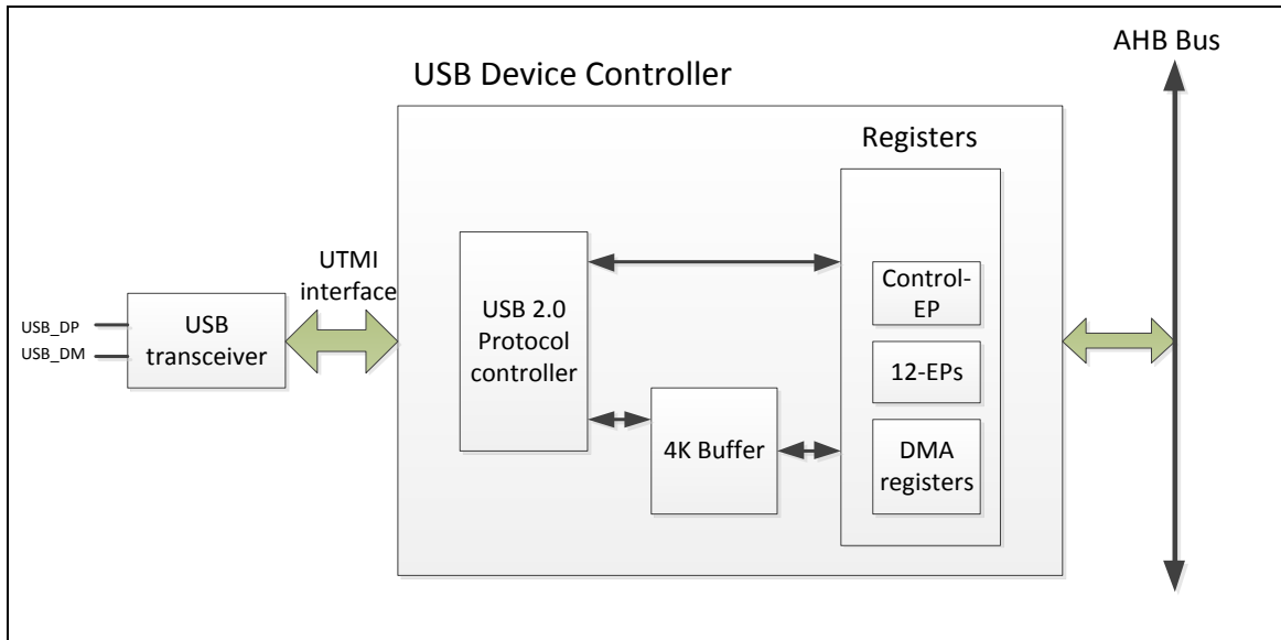
Figure 5.21-1 USB Device Controller Block Diagram
