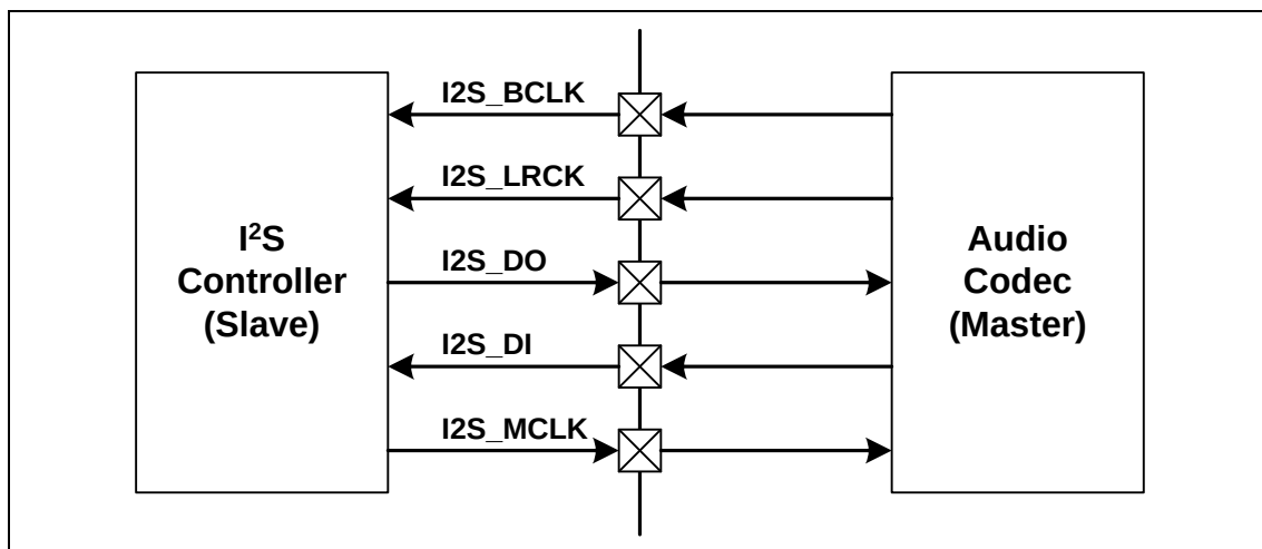
Figure 5.19-3 I 2 S Interface Signal of Slave Mode
