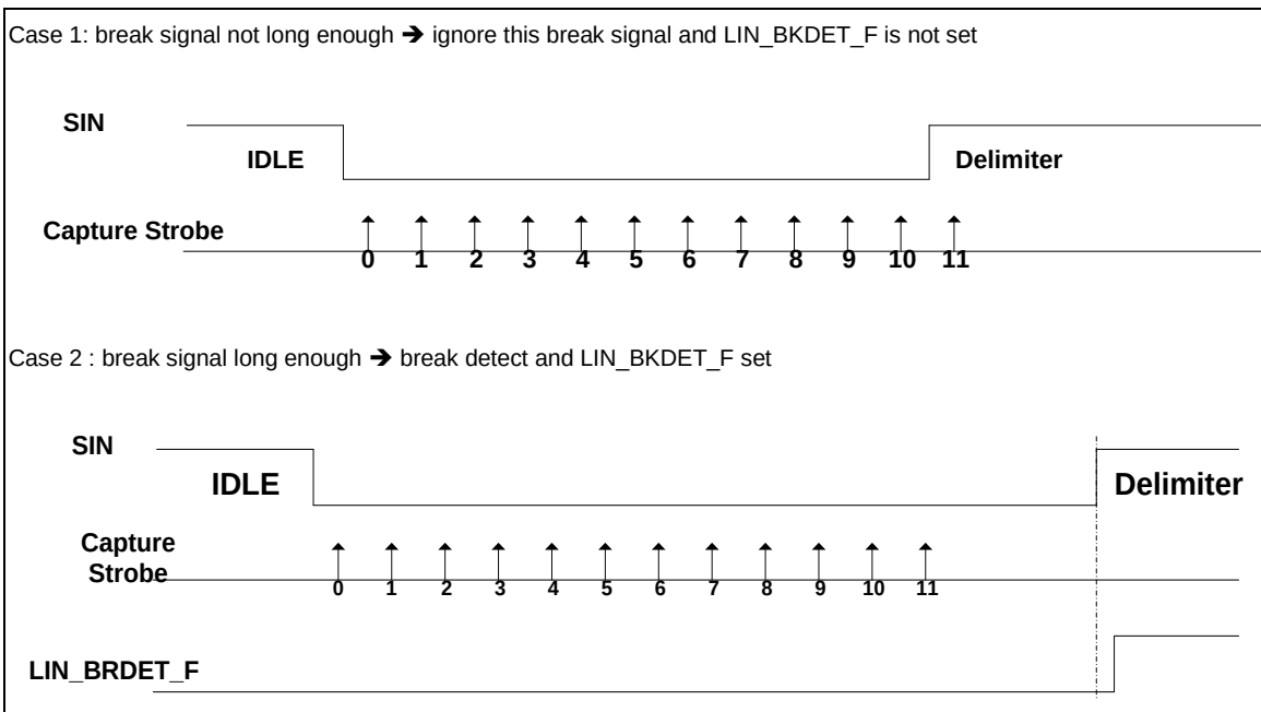
Figure 5.15-12 Break Detection in LIN Mode
