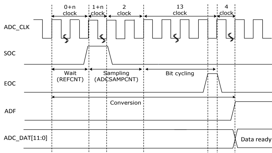
Figure 5.30-4 ADC Timing Diagram
