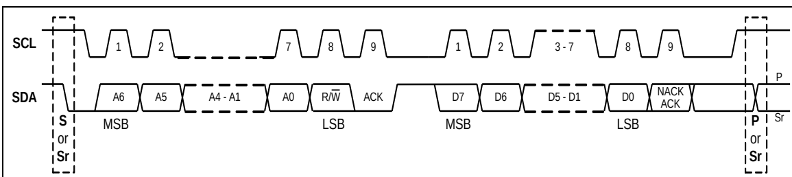
Figure 5.17-3 Data transfer on the I 2 C-bus
