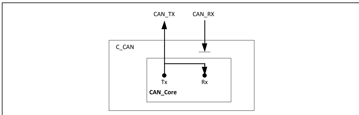
Figure 5.23-3 CAN Core in Loop Back Mode
