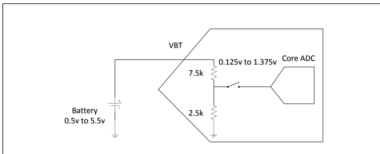
Figure 5.30-5 ADC Battery Voltage Detection Diagram
