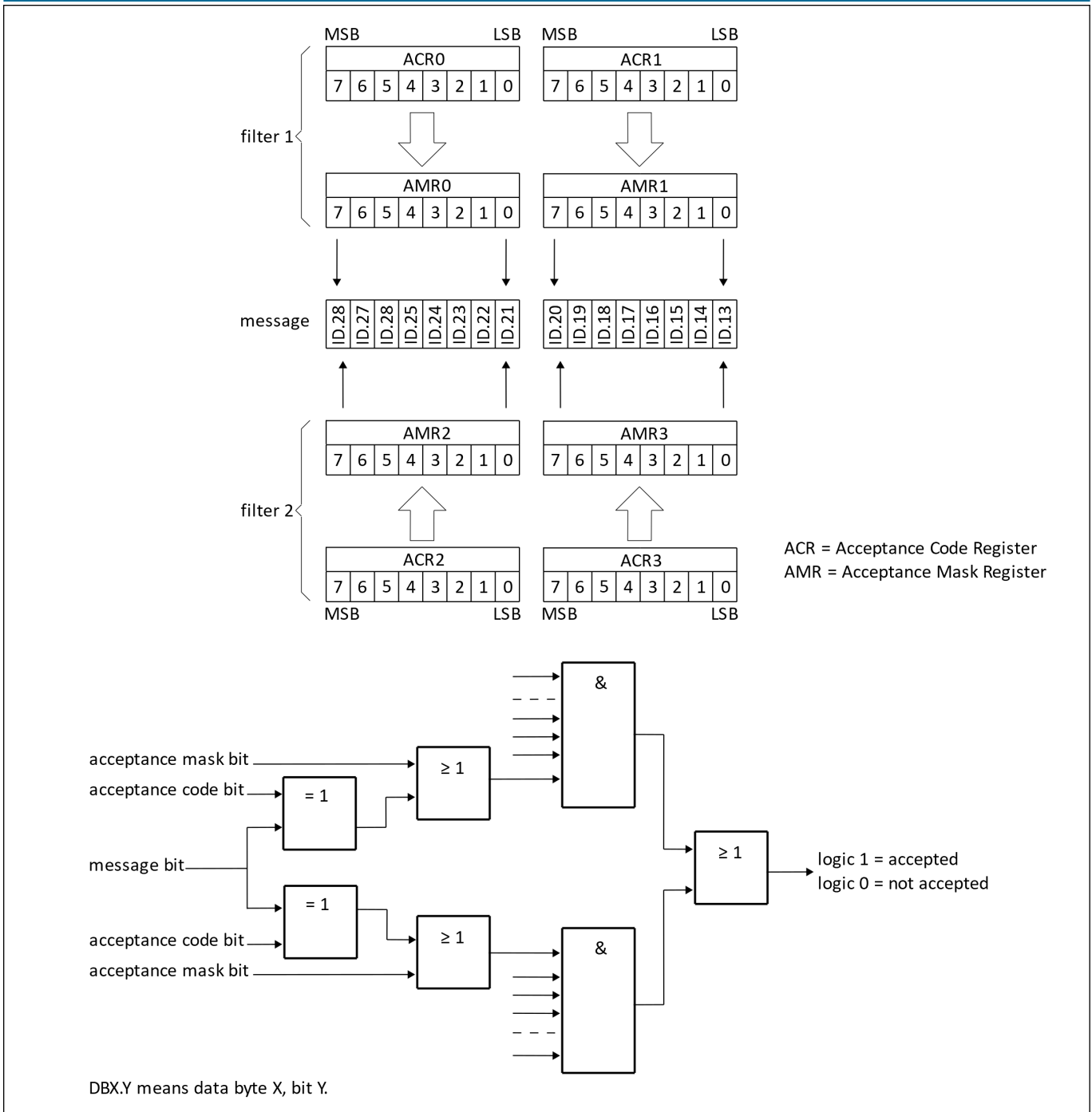
图 26.4: Dual filter configuration, receiving extended frame messages
