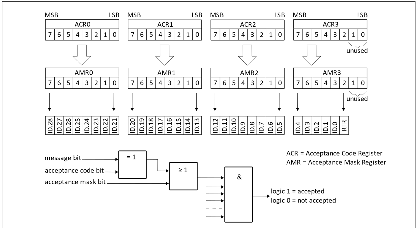
图 26.2: Single filter configuration, receiving extended frame messages
