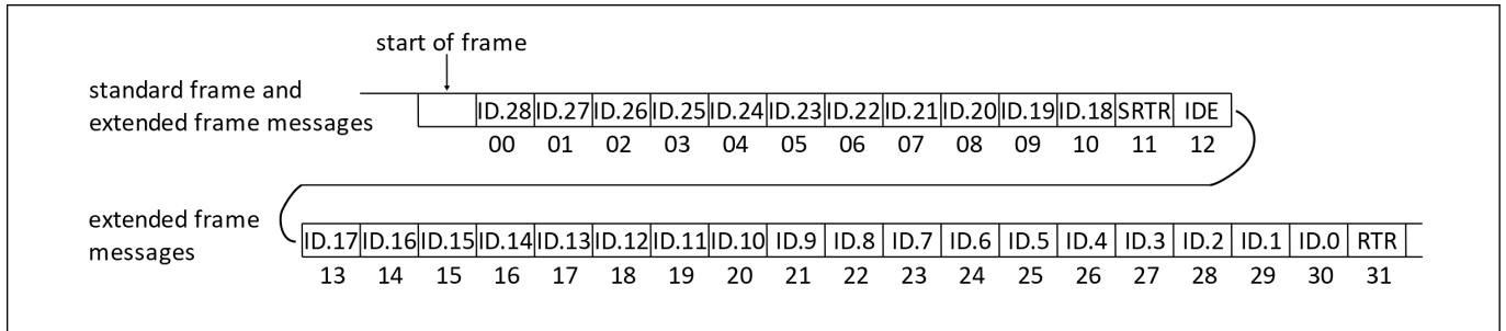
图 26.5: Arbitration lost bit number interpretation
