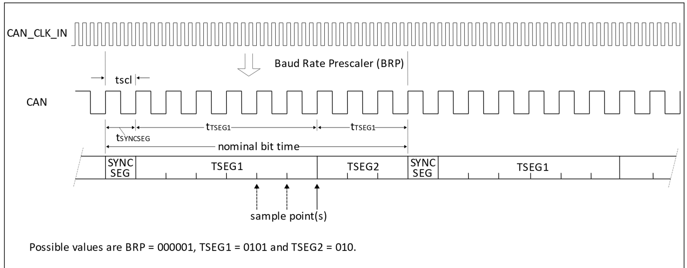
图 26.7: General structure of a bit period
