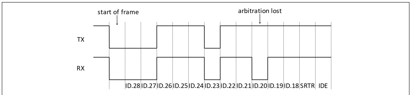
图 26.6: Example of arbitration lost bit number interpretation; result: ALC = 08
