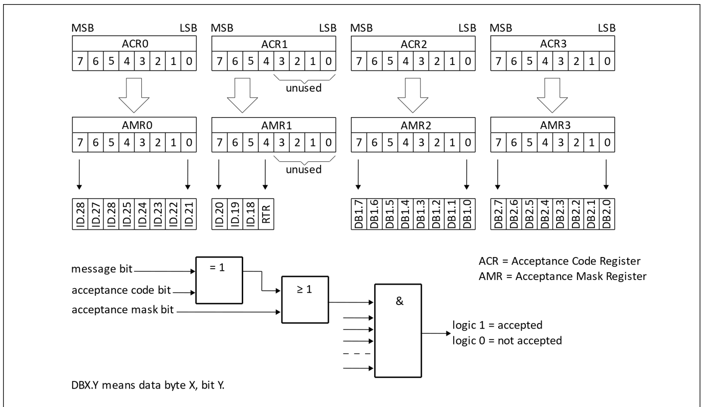
图 26.1: Single filter configuration, receiving standard frame messages
