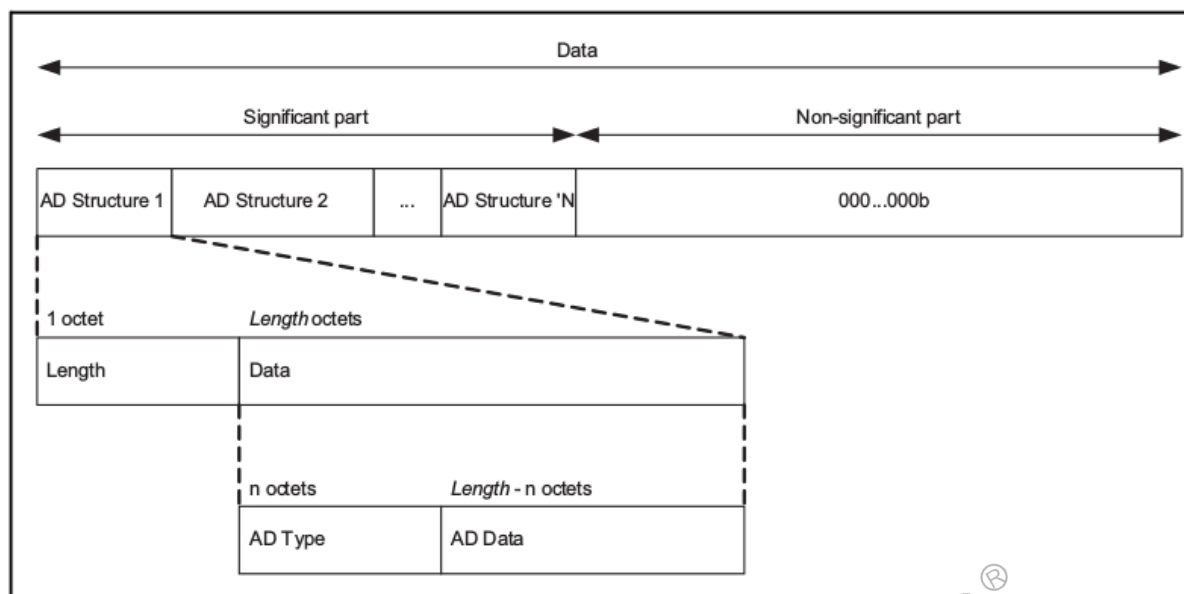
图 2-9: Advertising and Scan Response data format
